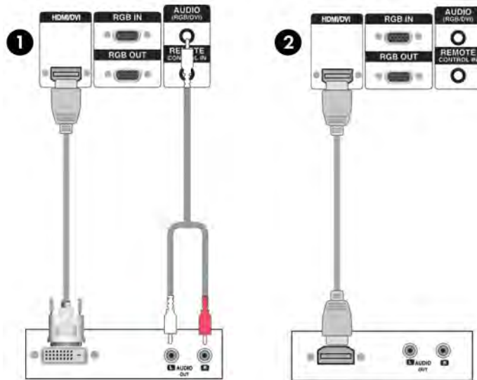
Figure 3-25 Connecting HDMI Input to VCR/DVD/Set-Top Box
