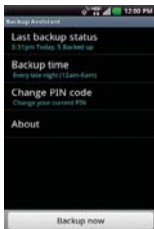
Settings screen
