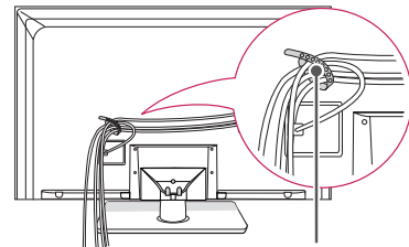
Cable holder
