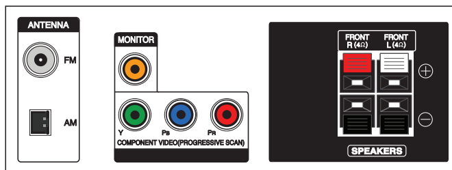
BACK PANEL
