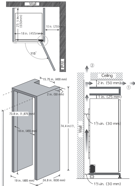
Built-In Installation
