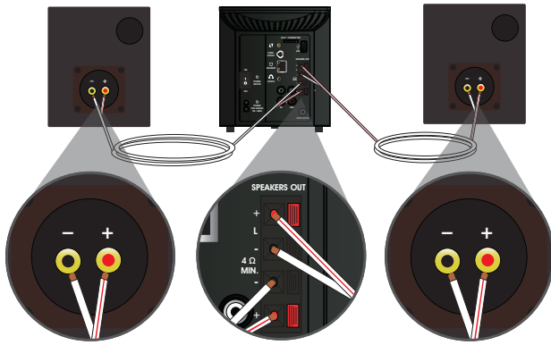
Speaker Connections
