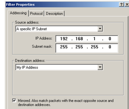
Figure C-8: Filters Properties
