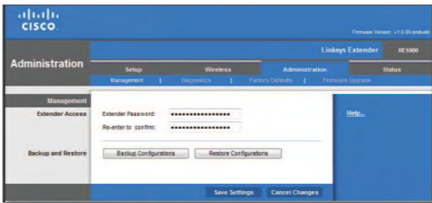
Administration > Management
