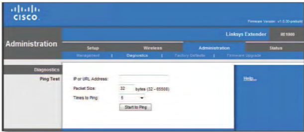
Administration > Diagnostics
