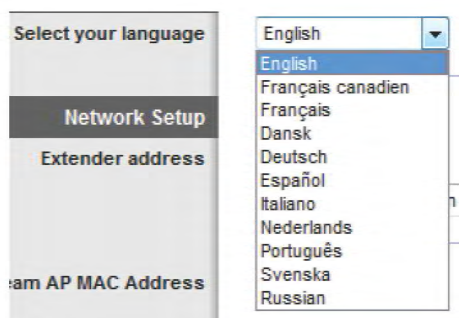
Setup > Languages
