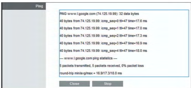
Diagnostics > Ping
