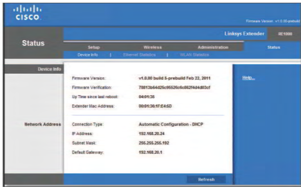
Status > Router
