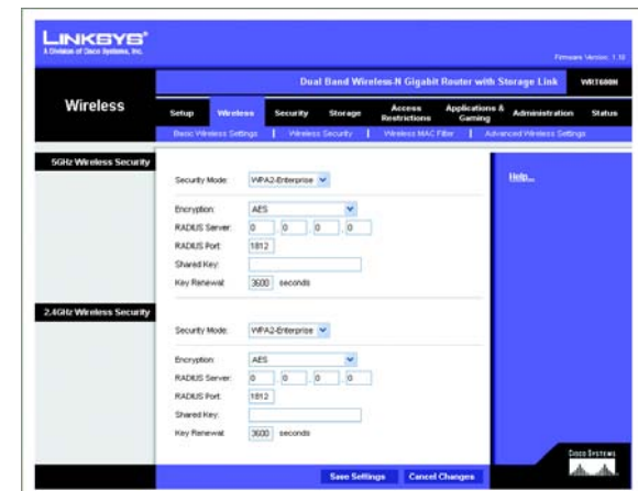
Figure 5-18: Wireless Security - WPA2-Enterprise
