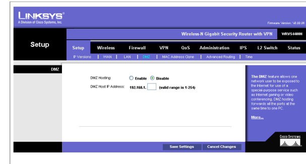
Figure 6-12: Setup - DMZ
