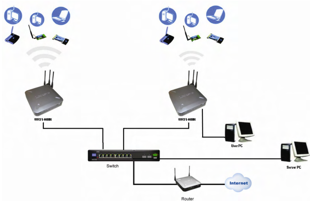
Figure 2-1: Example network
