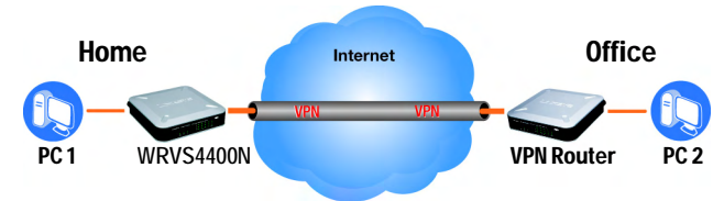
Figure 3-1: VPN Router to VPN Router
