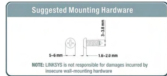
Figure 5-7: Mounting Dimensions
