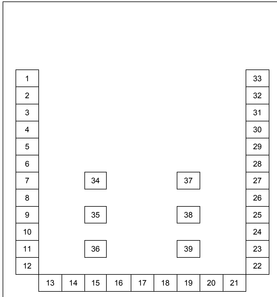
Figure 1 SaBLE-x Module Footprint (Viewed From Top)
