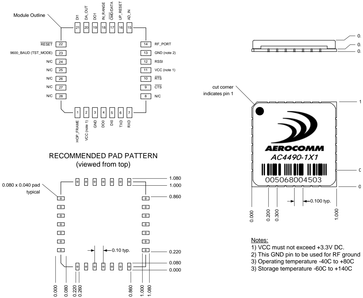
Figure 12: AC4490-1x1 Mechanical
