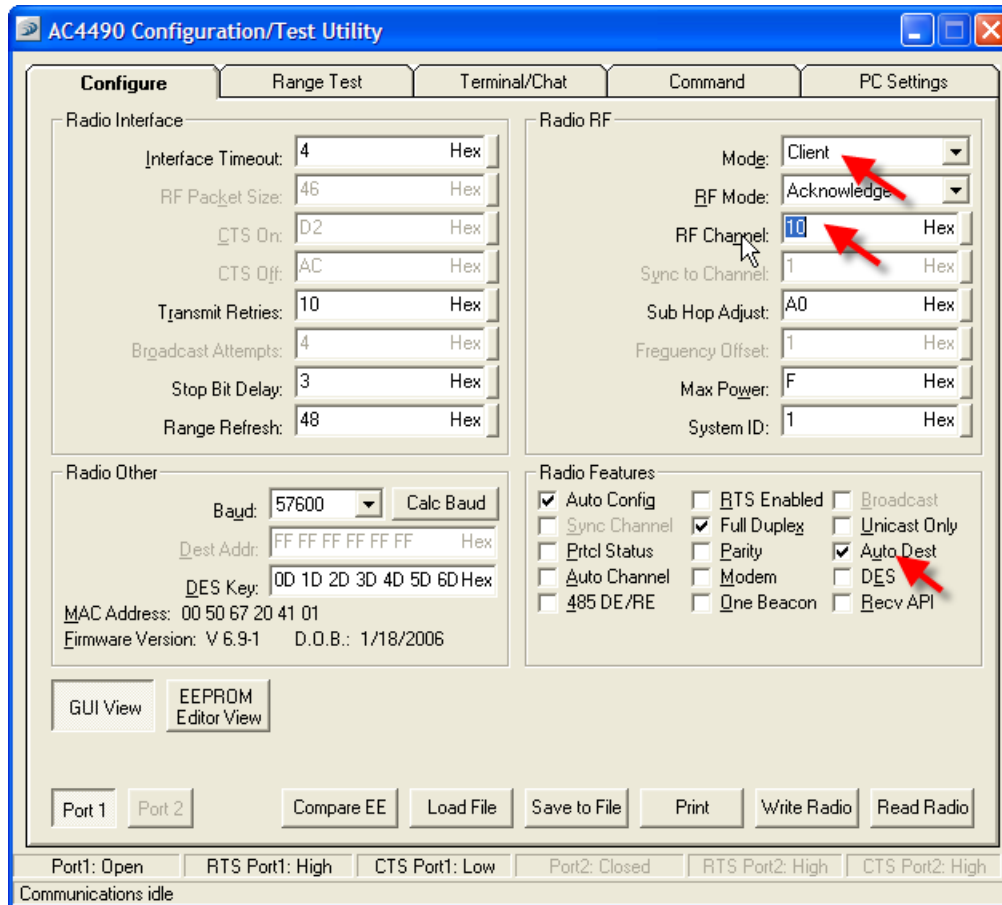
Figure 19: Client Settings
