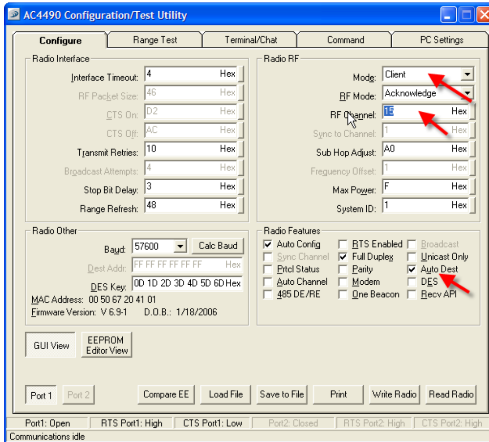
Figure 21: Client Settings
