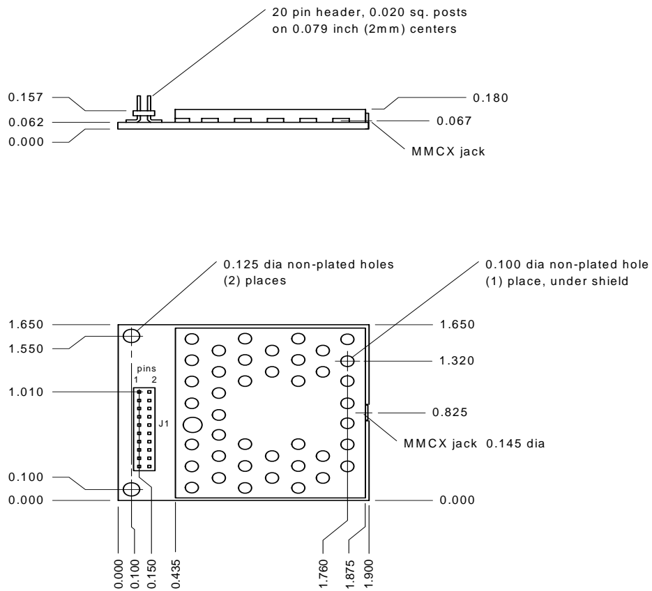
Figure 10: AC4490 (with MMCX connector) Mechanical
