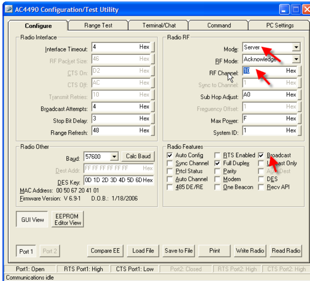
Figure 18: Hop Master Settings
