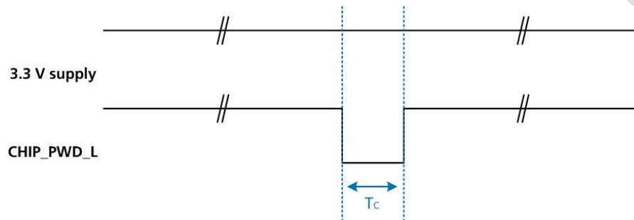
Figure 3: Reset timing
