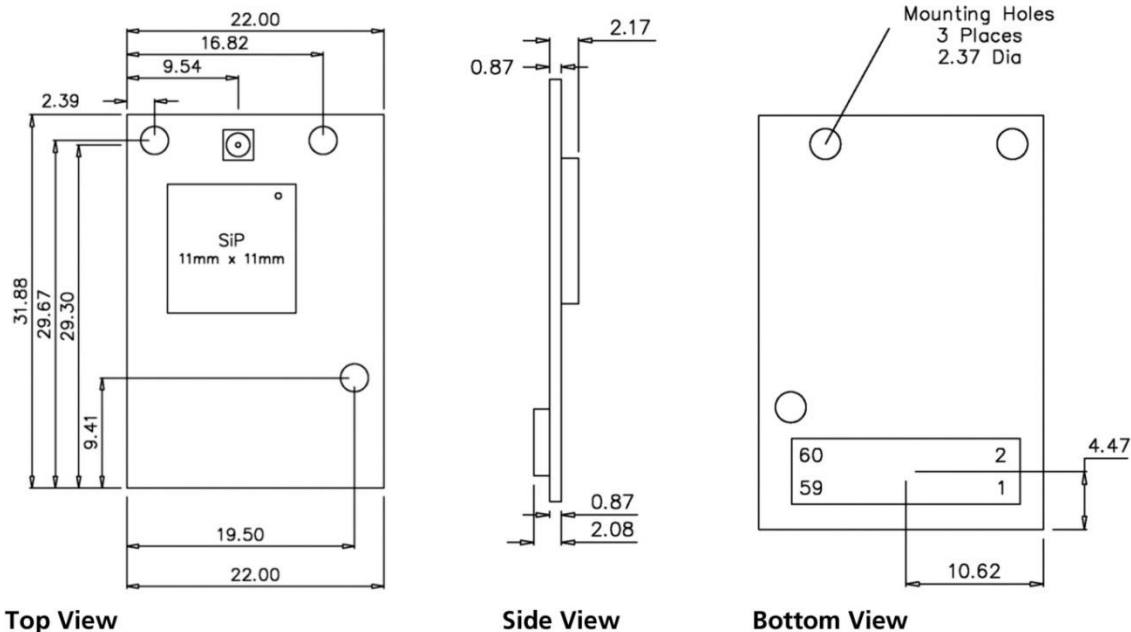
Figure 4: Mechanical Drawing
