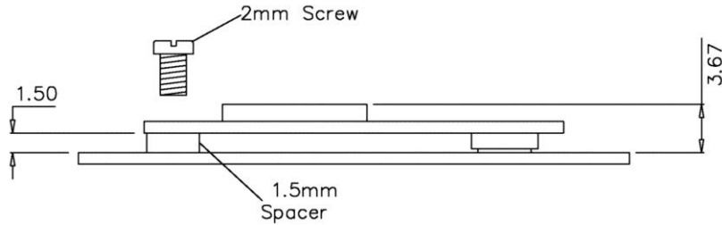
Figure 6: Mounting Recommendations
