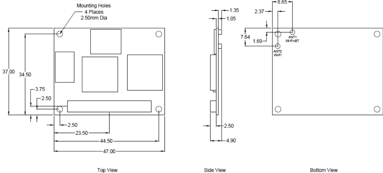
Figure 1: WB50NBT mechanical drawing
