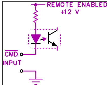
Figure 3 TX_OFF, RESET, and VOR Remote Controls
