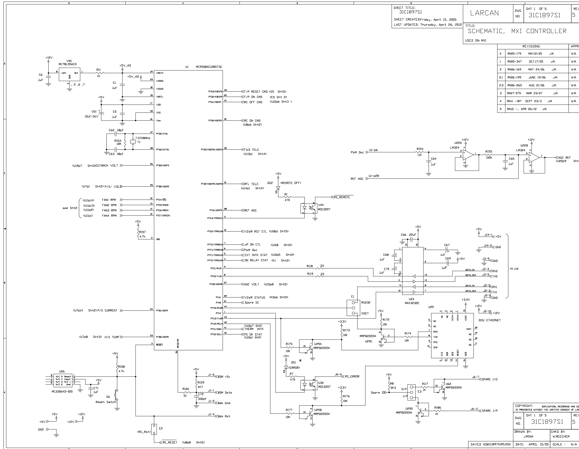
Figure 6 MXi Controller Board Schematic 31C1897S1 sht1
