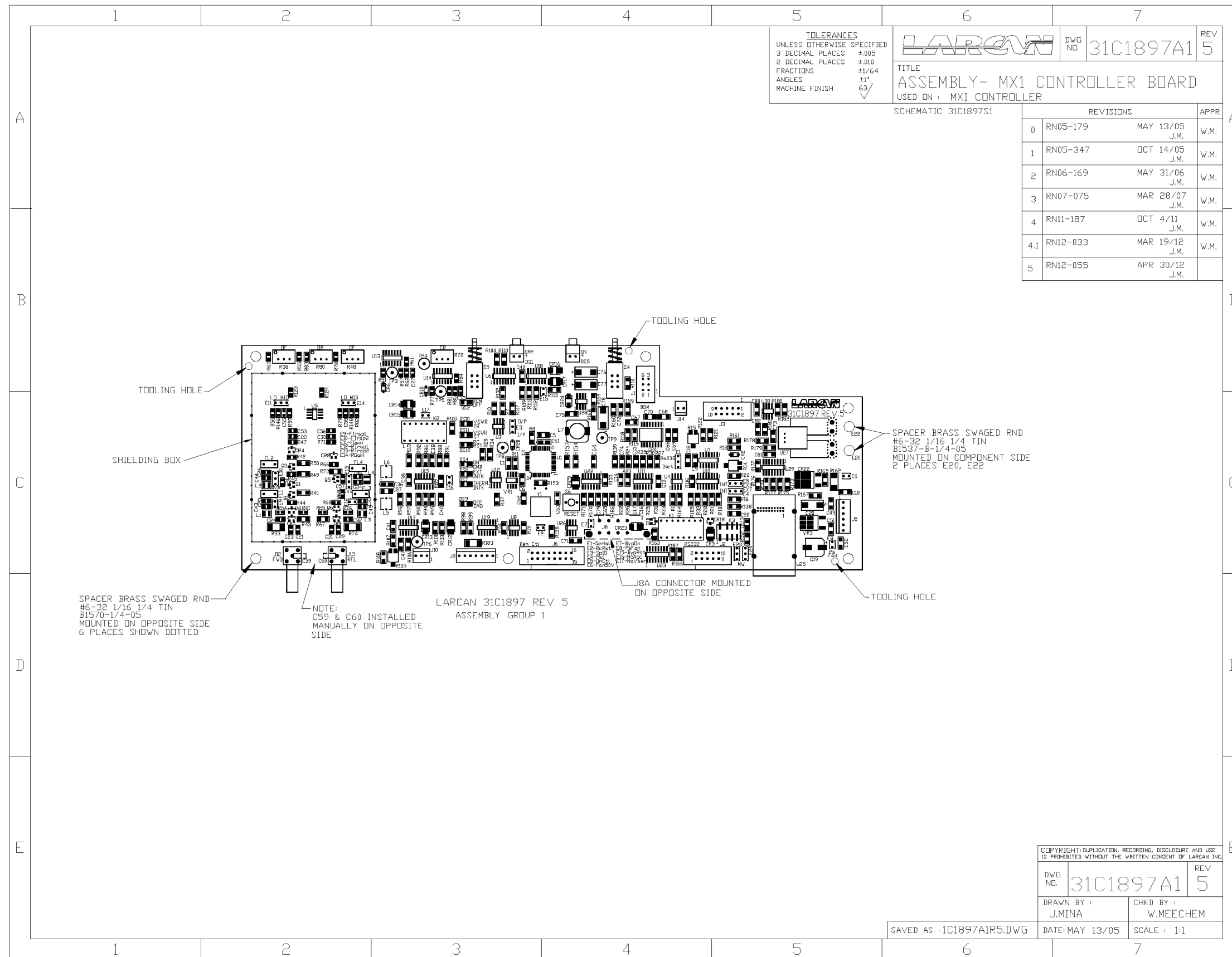
Figure 5 MXi Controller Board Assembly Diagram 31C1897A1
