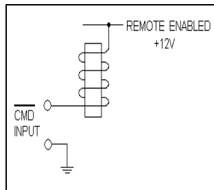
Figure 4 TX_ON Remote Control
