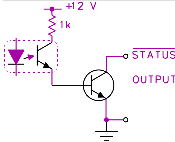
Figure 2 Status Outputs
