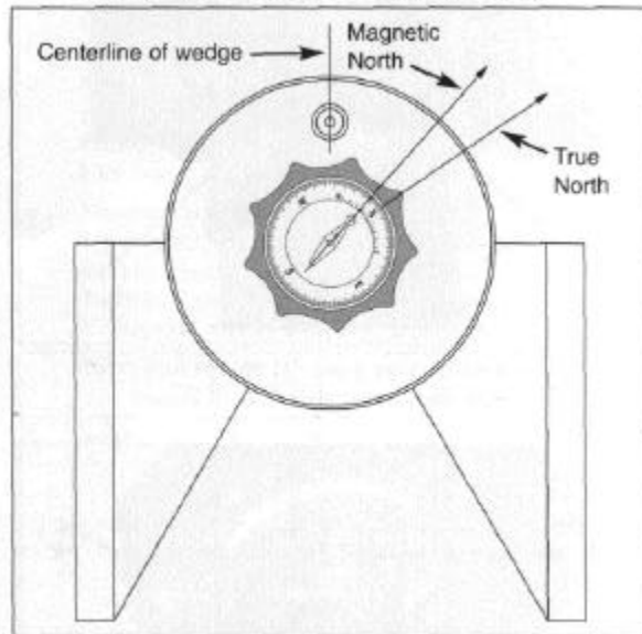
Fig. 18: Equatorial Wedge.
