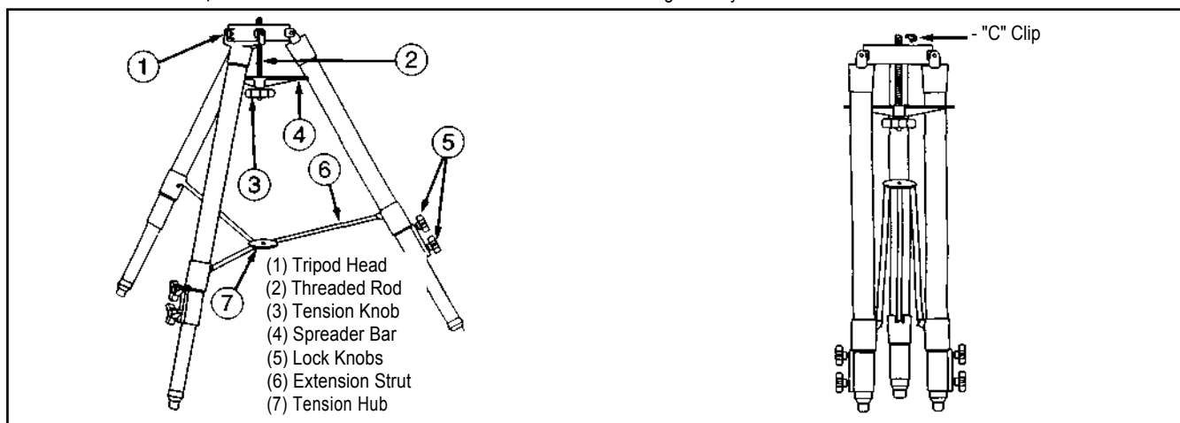
Fig. 1: Field Tripod
