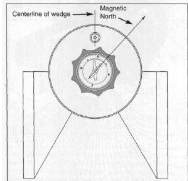
Fig. 17: Equatorial Wedge.
