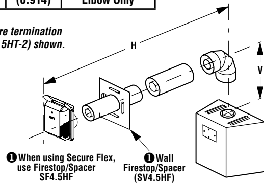
Figure 37 - Top Vent - ONE 90 DEGREE ELBOW - ELBOW CONNECTION AT APPLIANCE
