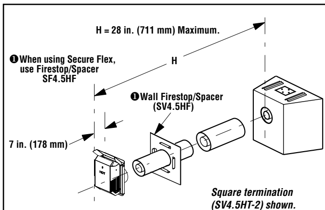
Figure 36 - Rear Vent - NO ELBOWS - Square Horizontal Termination (SV4.5HT-2)
