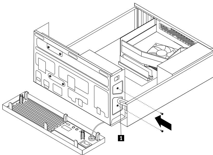
Figure 66. Installing the optical drive
