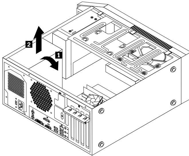
Figure 18. Removing the power supply assembly
