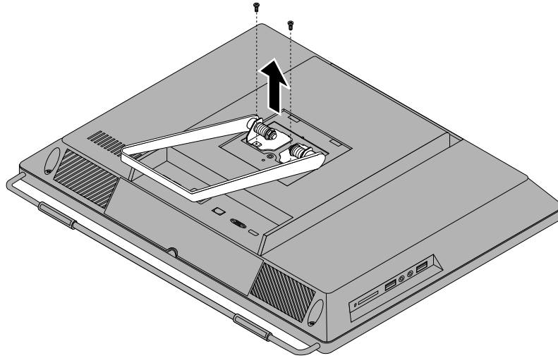
Figure 8. Removing the system stand
