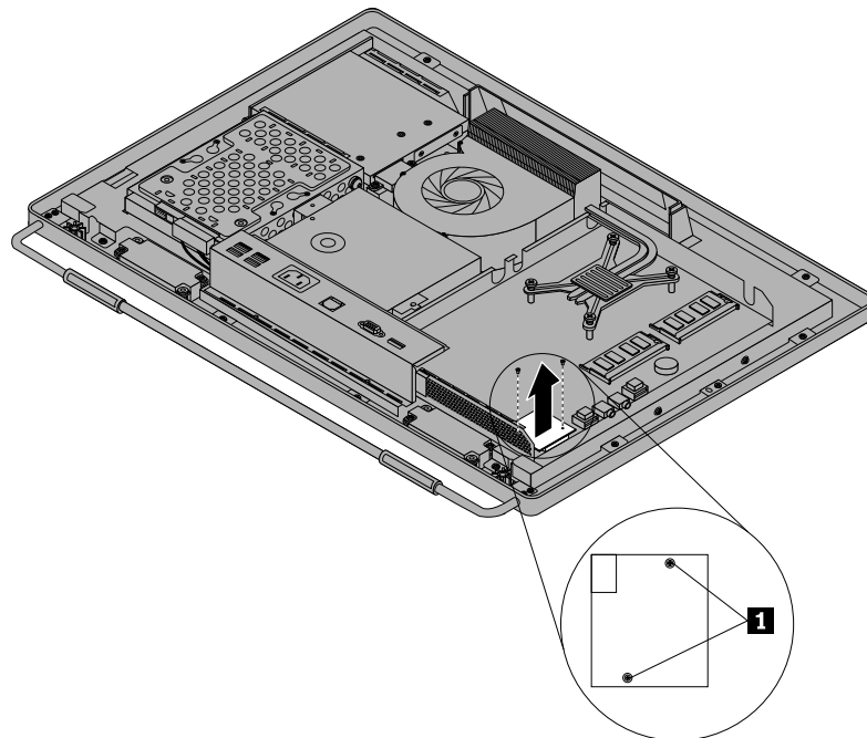
Figure 30. Removing the card reader
