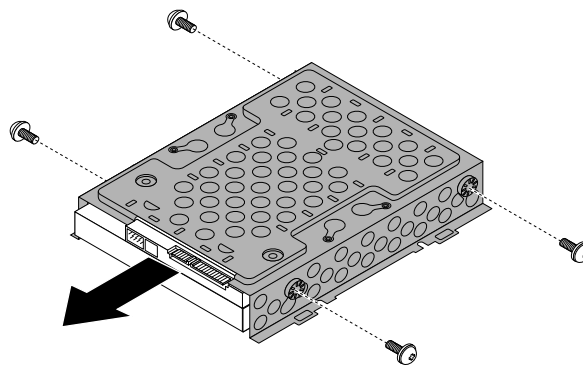
Figure 15. Removing the hard disk drive out of the bracket
