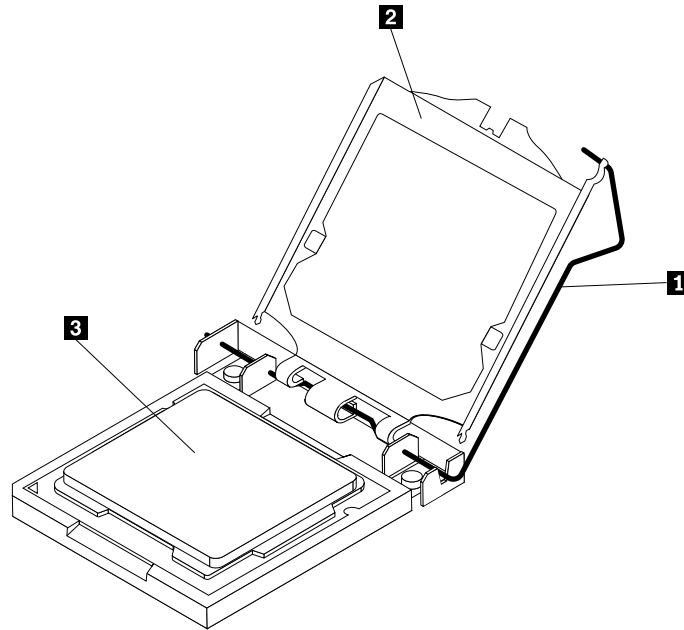
Figure 26. Opening the retainer to access the microprocessor
