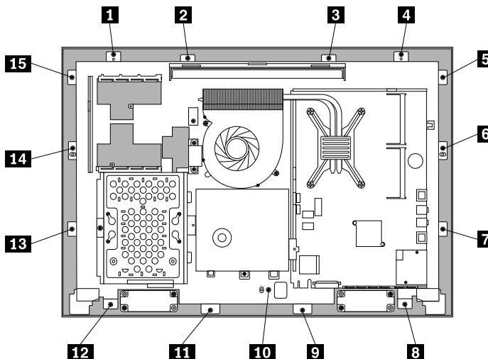
Figure 42. Removing all the 15 screws that secure the computer main bracket to the front bezel
