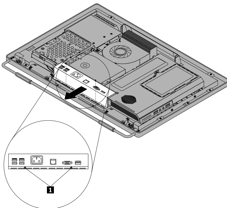
Figure 20. Removing the two screws that secure the rear I/O assembly
