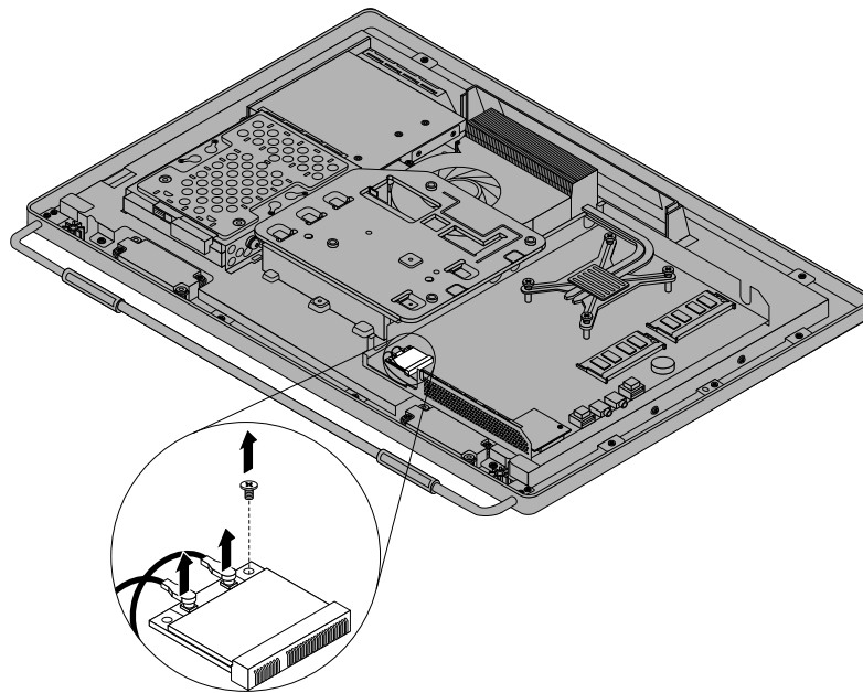
Figure 46. Removing the screw that secures the WI-FI card to the system board
