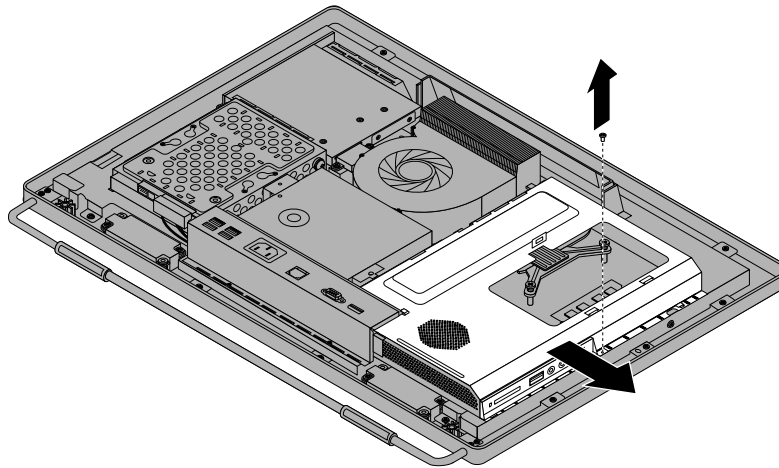
Figure 22. Removing the system board shield
