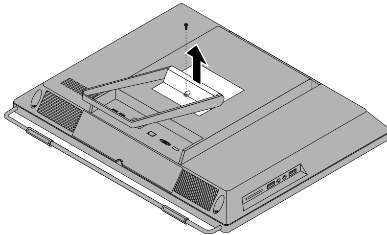
Figure 5. Removing the system stand hinge cover
