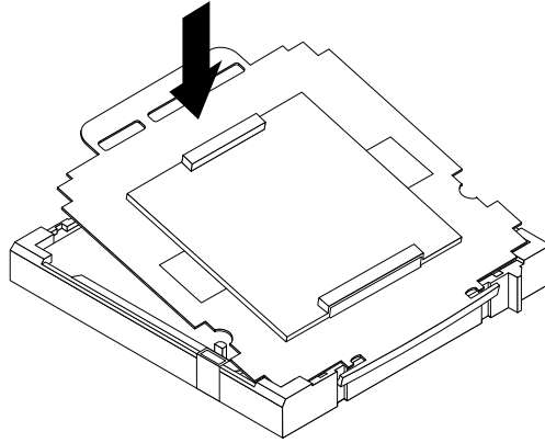
Figure 39. Installing one side of the socket cover into the microprocessor socket
