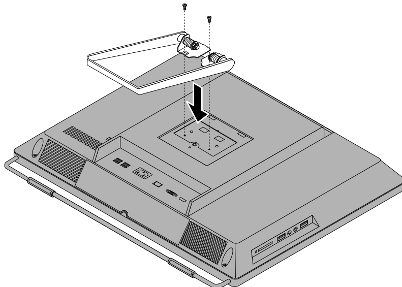
Figure 9. Reinstalling the system stand
