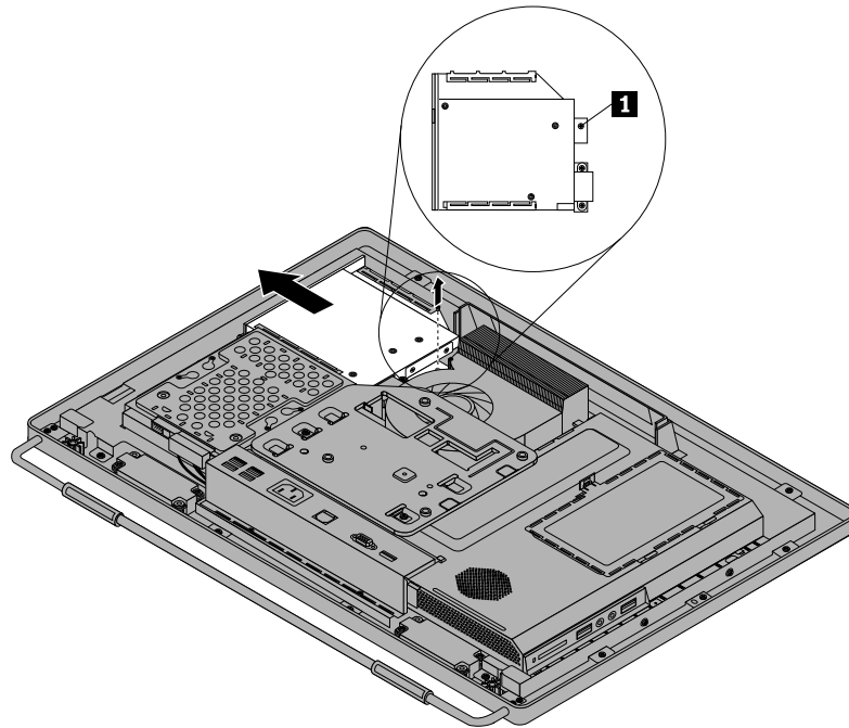
Figure 16. Removing the optical drive
