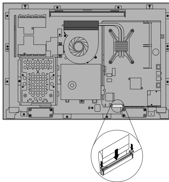
Figure 45. Reconnect the LCD panel cable to the system board
