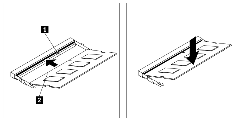
Figure 35. Installing a memory module
