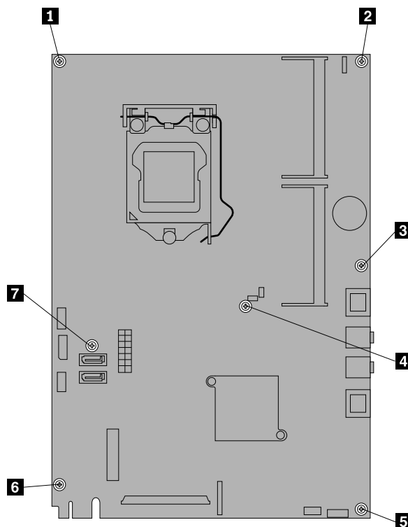
Figure 38. Removing the seven screws that secure the system board to the main bracket
