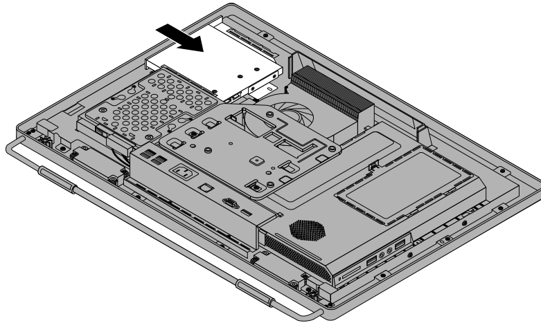
Figure 17. Installing the optical drive
