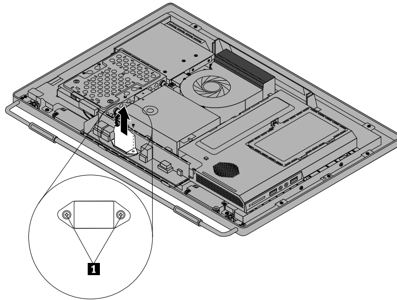
Figure 21. Removing the power cord connector
