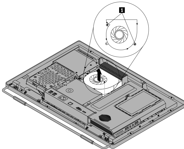
Figure 24. Removing the microprocessor fan
