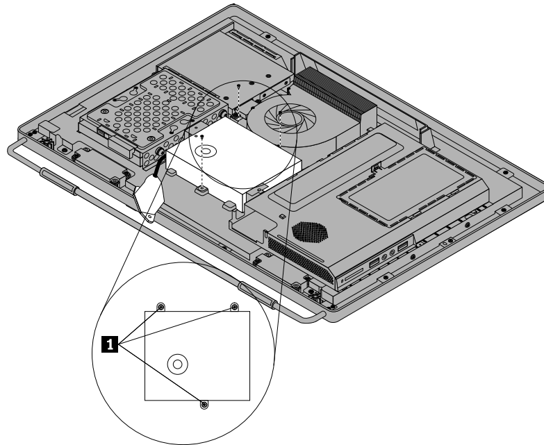
Figure 23. Removing the three screws that secure the power supply
