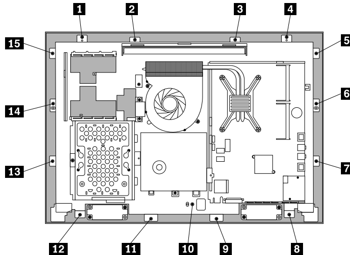
Figure 44. Reinstalling all the 15 screws that secure the computer main bracket to the front bezel
