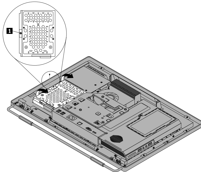
Figure 13. Removing the screw that secures the hard disk drive
