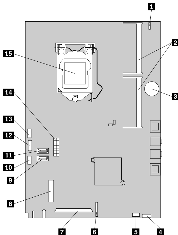
Figure 4. System board part and connector locations
