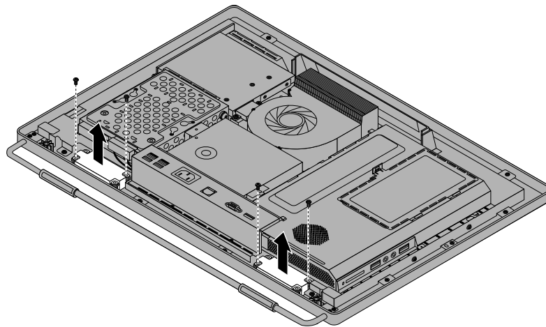
Figure 36. Removing the internal speakers
