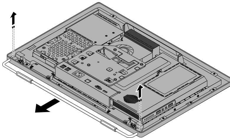
Figure 10. Removing the frame stand
