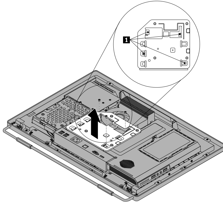
Figure 19. Removing the VESA mount bracket
