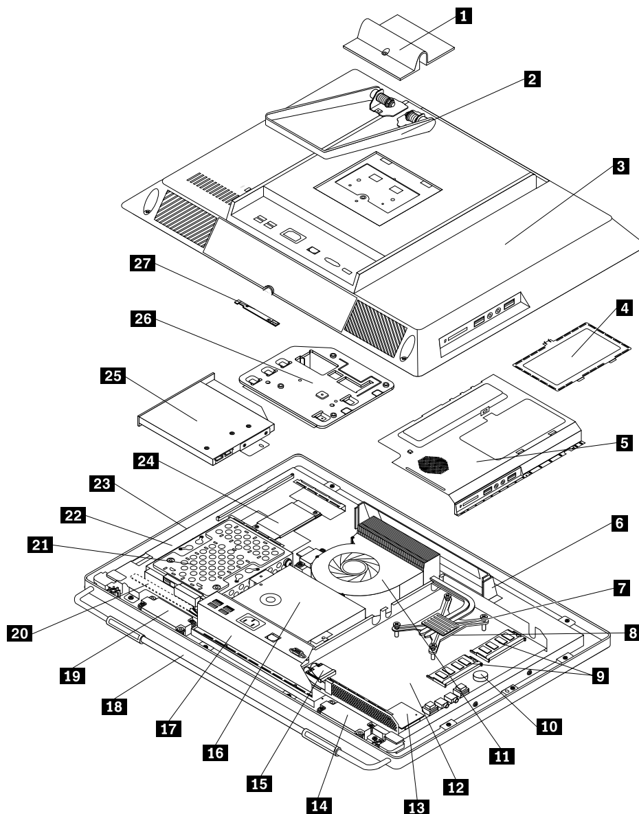
Figure 3. FRU locations
