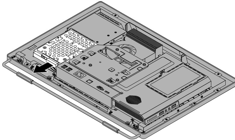
Figure 14. Removing the hard disk drive
