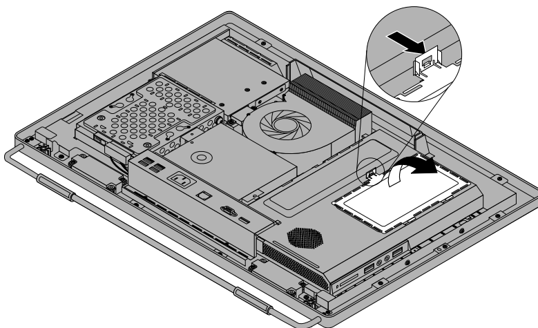
Figure 31. Opening the system board shield window
