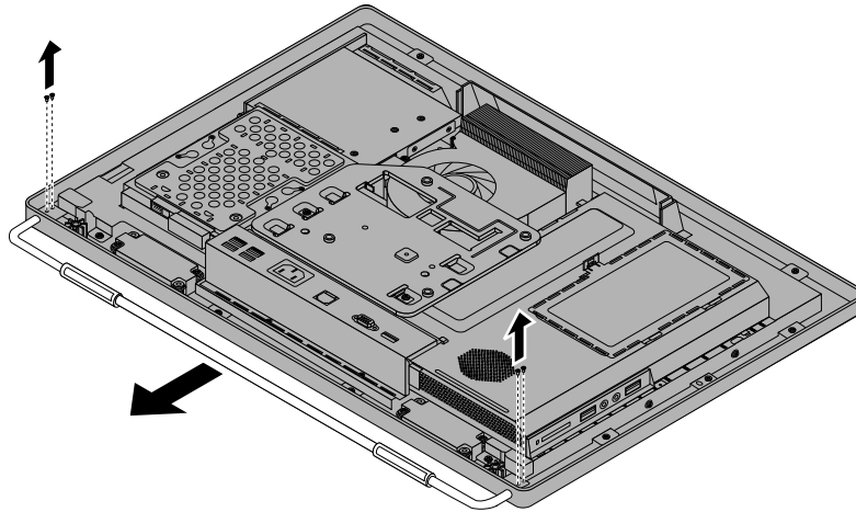
Figure 40. Removing the frame stand
