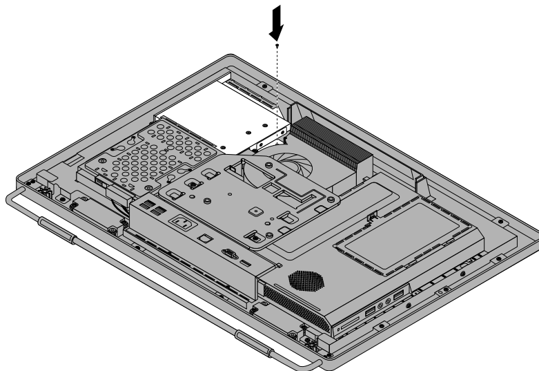
Figure 18. Installing the screw to secure the optical drive
