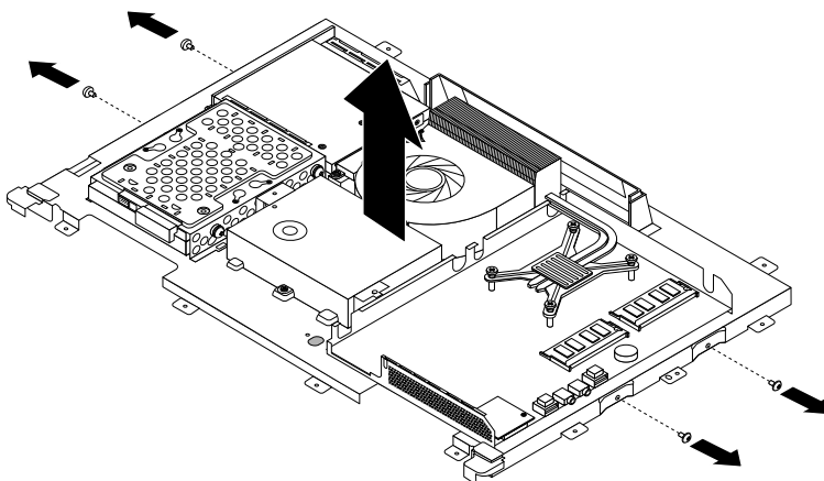
Figure 43. Removing the four screws that secure the LCD panel
