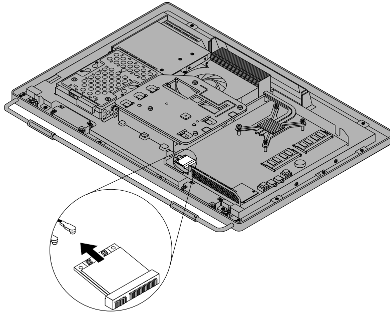
Figure 47. Removing the WI-FI card
