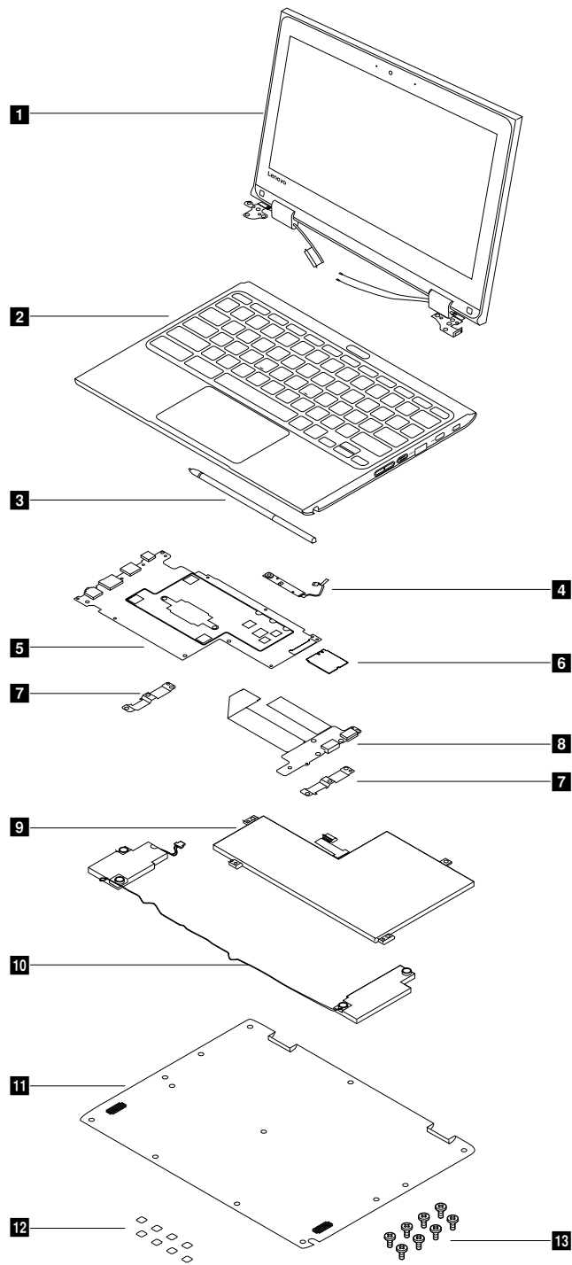
Figure 1. 500e Chromebook exploded view
