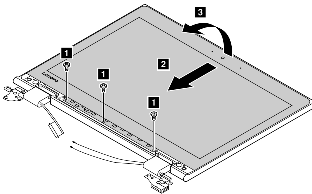
Figure 6. Remove 4 screws and lift up the LCD panel
