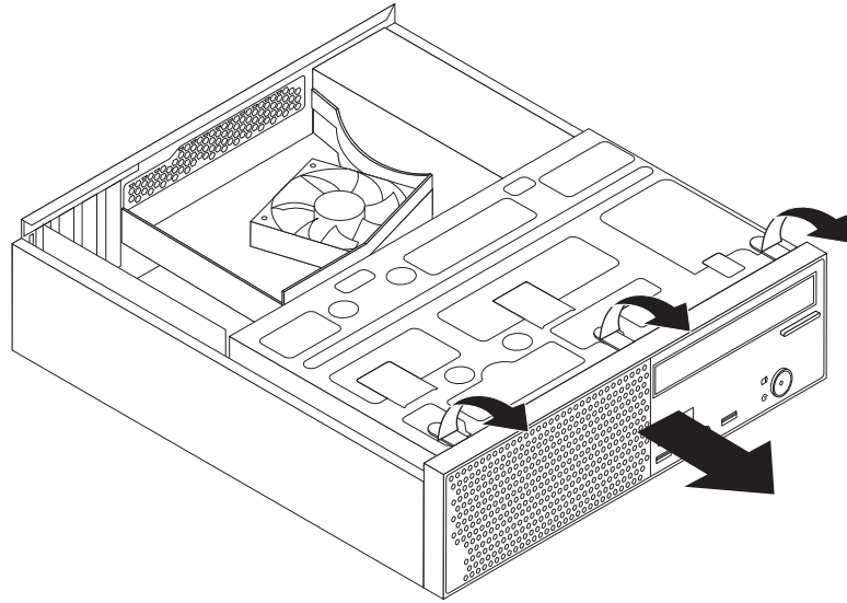
Figure 7. Removing the front bezel
