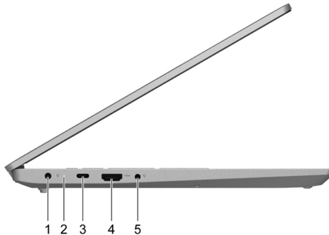
Figure 4. IdeaPad 5 (14", 05) and Lenovo Ducati 5- left view
