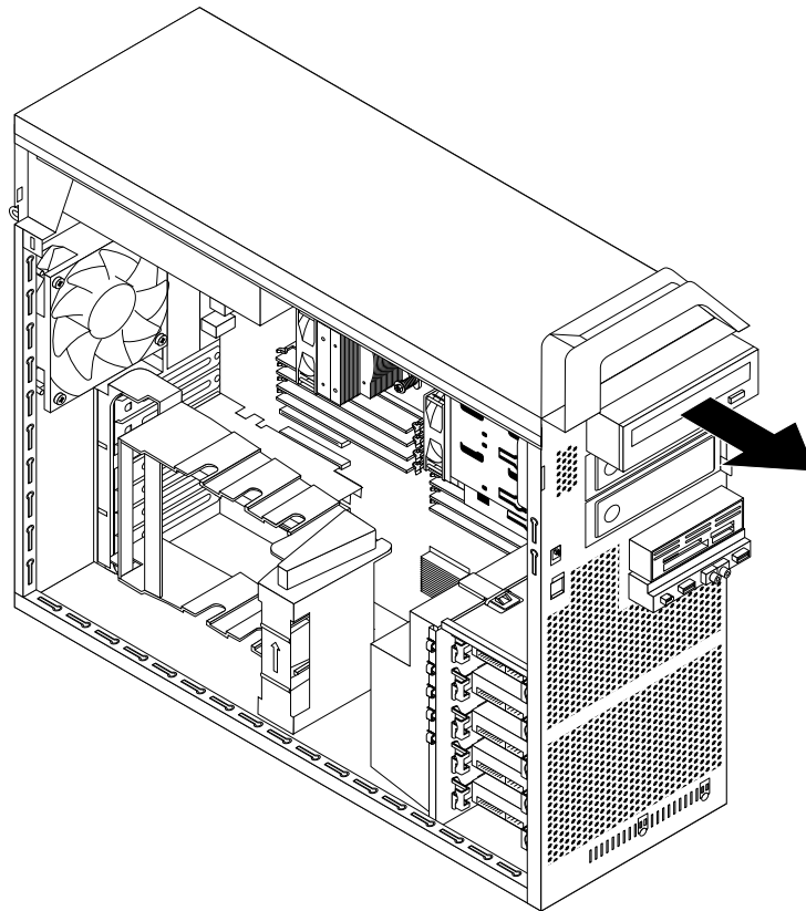
Figure 19. Installing the optical drive
