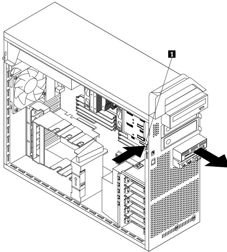
Figure 21. Removing the card reader
