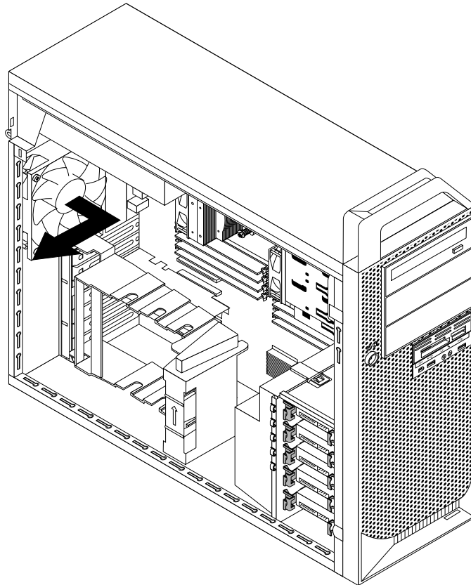
Figure 28. Removing the rear fan assembly
