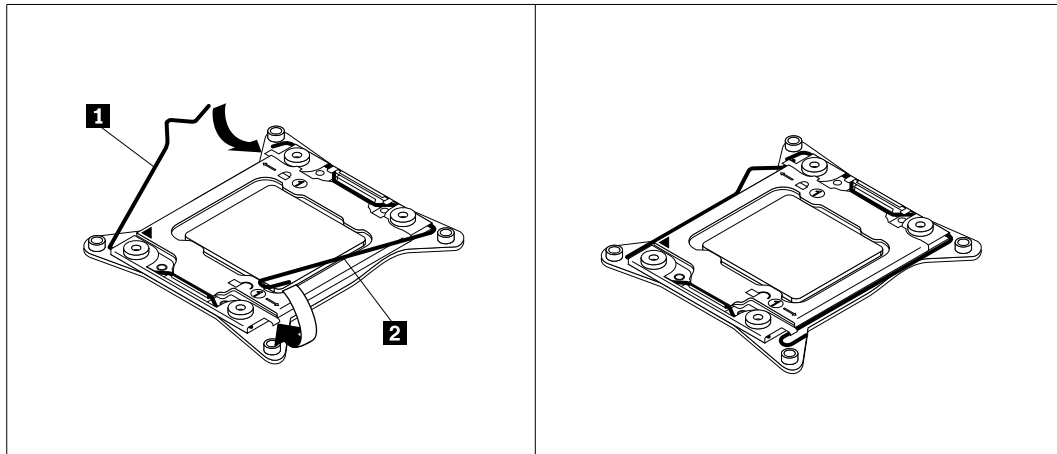
Figure 45. Securing the microprocessor in the socket
