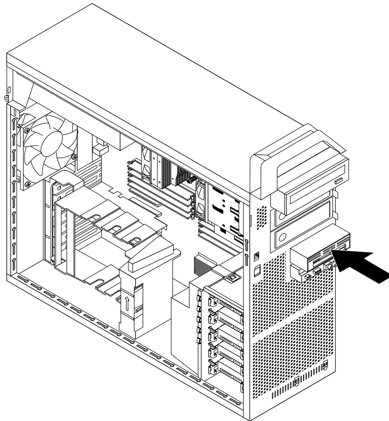
Figure 23. Installing the card reader
