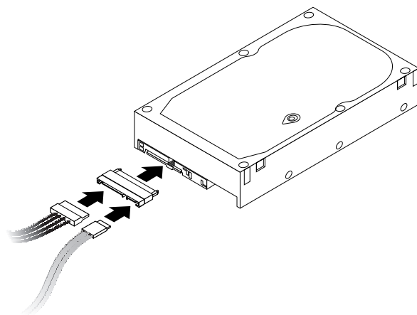
Figure 34. Connecting SAS cables to SAS-to-SATA conversion adapter
