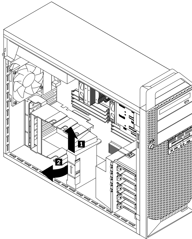
Figure 8. Opening the PCI card retainer
