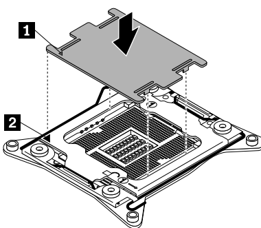
Figure 56. Installing the microprocessor socket cover
