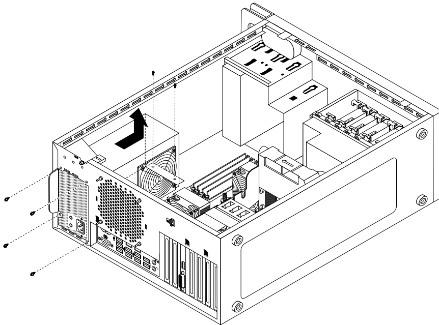
Figure 57. Removing six screws that secure the power supply assembly
