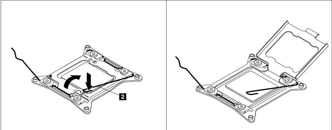
Figure 47. Opening the microprocessor retainer
