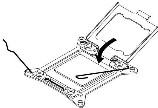
Figure 44. Closing the microprocessor retainer
