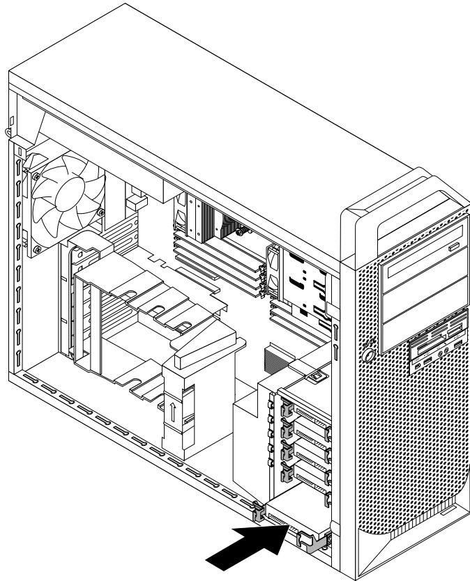
Figure 33. Installing the hard disk drive
