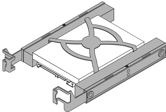
Figure 32. Installing 2.5-inch to 3.5-inch converter bracket before installing the outer bracket
