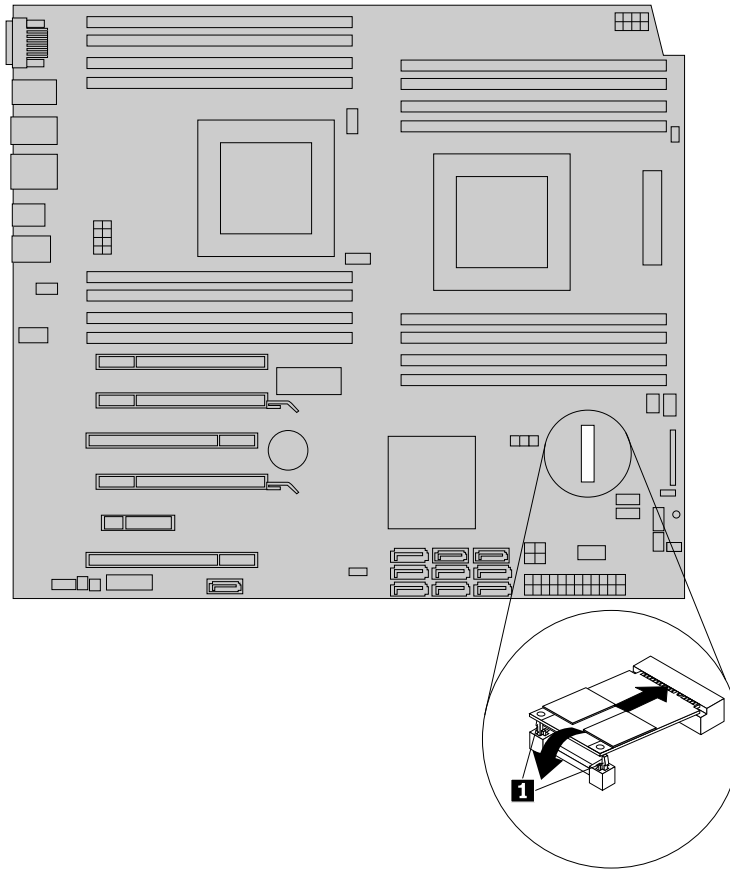
Figure 11. Installing an mSATA solid-state drive
