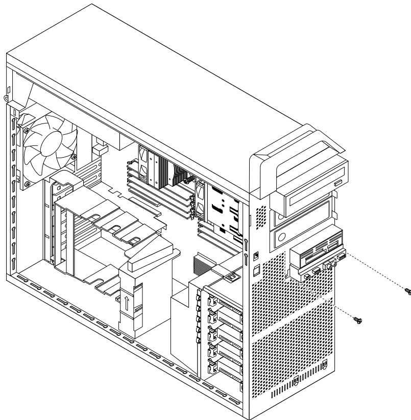
Figure 37. Removing the two screws that secure the front audio and USB assembly to the chassis
