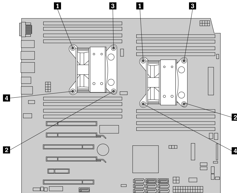
Figure 26. Removing the heat sink and fan assembly
