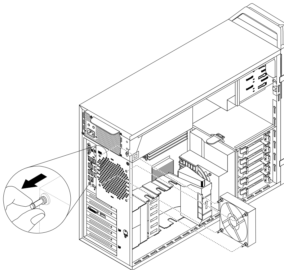
Figure 29. Installing the rear fan assembly
