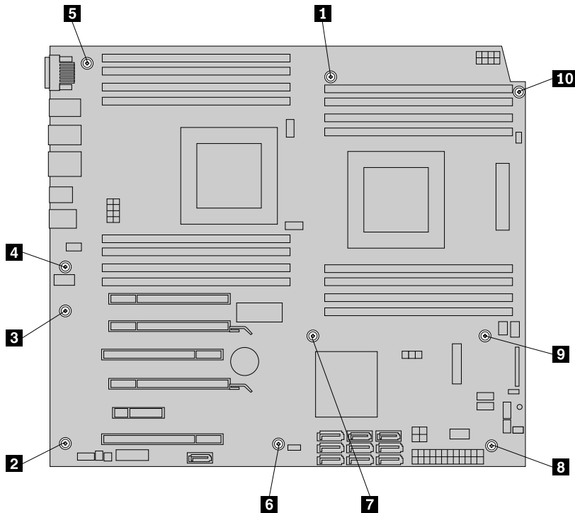
Figure 53. Removing the ten screws that secure the system board to the chassis
