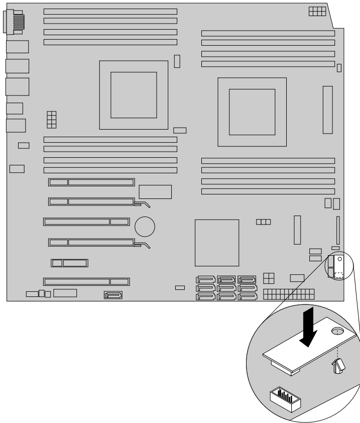
Figure 36. Installing a new hard disk drive enablement module
