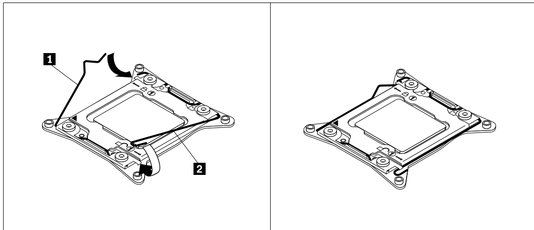
Figure 52. Securing the microprocessor in the socket
