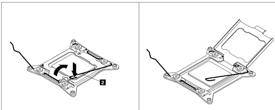
Figure 40. Opening the microprocessor retainer
