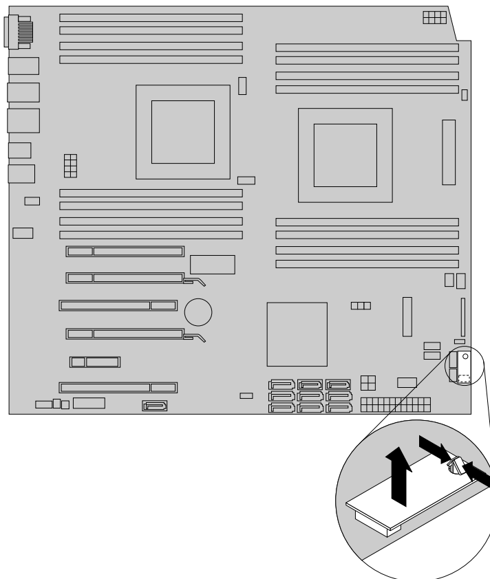
Figure 35. Removing the hard disk drive enablement module
