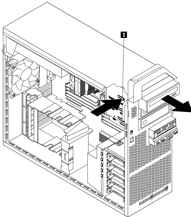
Figure 17. Removing the optical drive
