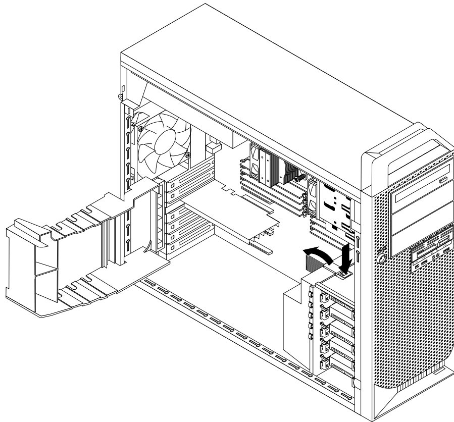
Figure 27. Removing the hard disk drive fan assembly
