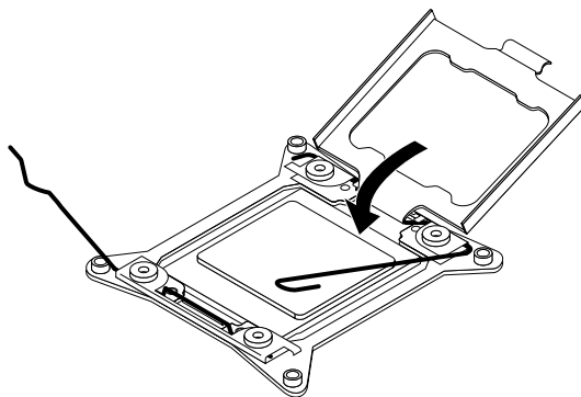
Figure 54. Closing the microprocessor retainer
