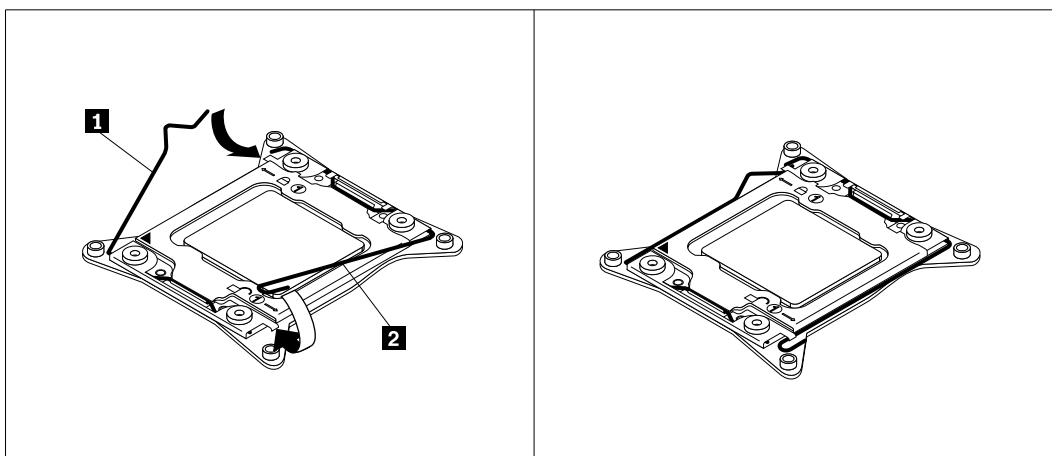
Figure 55. Securing the microprocessor in the socket
