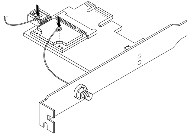
Figure 37. Installing the WiFi antenna cables
