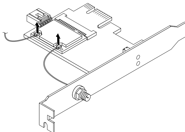
Figure 33. Removing the WiFi antenna cables
