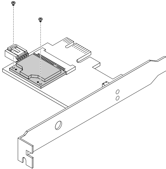
Figure 34. Removing the screws that secure the WiFi card module
