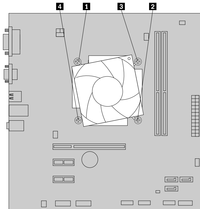
Figure 27. Removing the heat sink and fan assembly
