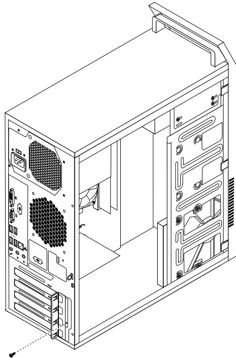
Figure 12. Removing the screw that secures the PCI card latch
