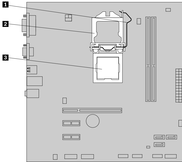
Figure 28. Accessing the microprocessor
