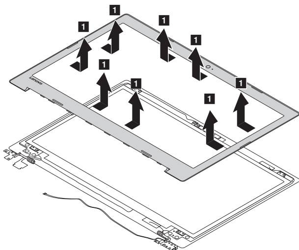
Figure 12. Removal steps of LCD unit (continued)
