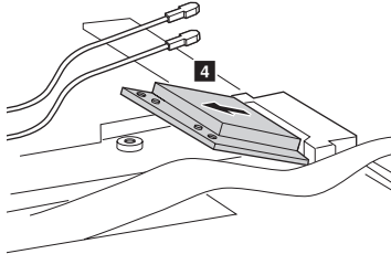
Figure 4. Removal steps of PCI Express Mini Card for wireless LAN/WAN (continued)
