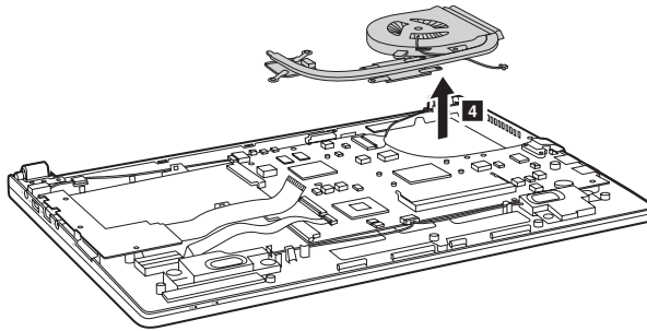
Figure 5. Removal steps of fan assembly and heat sink assembly (continued)
