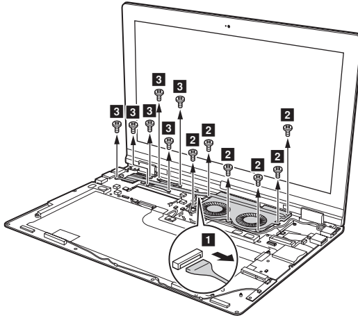
Figure 7. Removal steps of fan assembly and heat sink assembly
