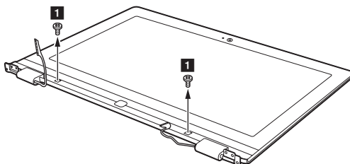
Figure 11. Removal steps of LCD front bezel
