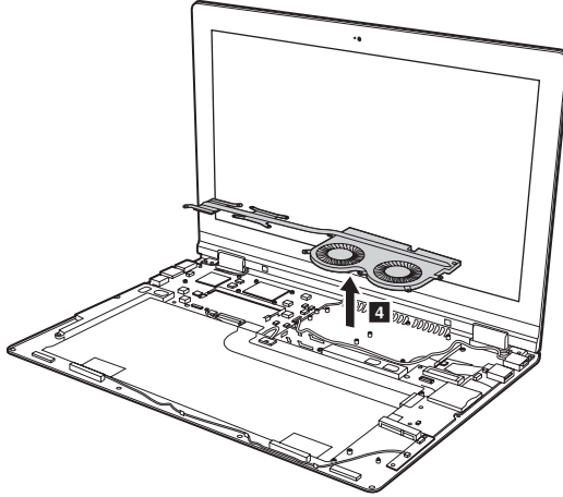
Figure 7. Removal steps of fan assembly and heat sink assembly (continued)
