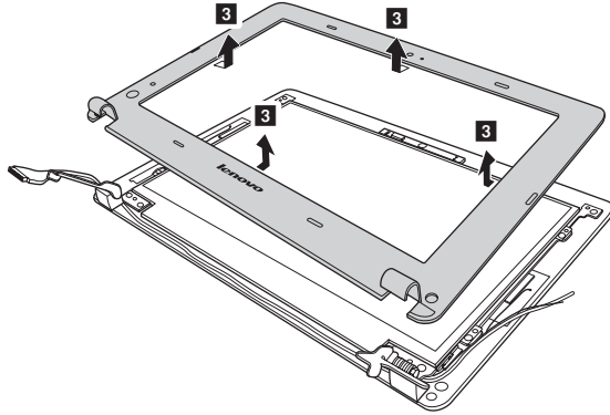
Figure 11. Removal steps of LCD front bezel (continued)
