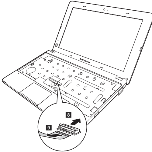
Figure 8. Removal steps of system board (continued)
