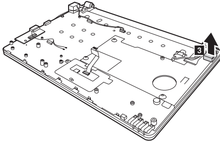
Figure 10. Removal steps of base cover, speakers, power assembly and USB board (continued)
