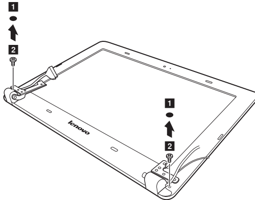
Figure 11. Removal steps of LCD front bezel
