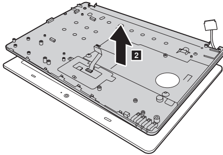
Figure 9. Removal steps of LCD unit (continued)
