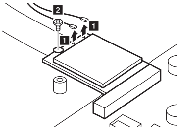
Figure 6. Removal steps of PCI Express Mini Card for wireless LAN/WAN
