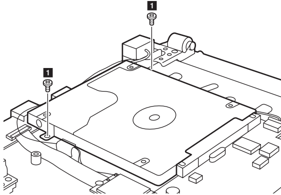
Figure 5. Removal steps of hard disk drive
