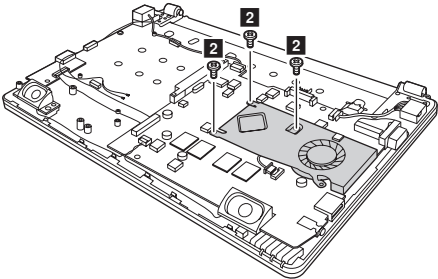
Figure 7. Removal steps of fan assembly and heat sink assembly (continued)
