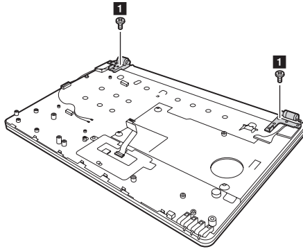
Figure 9. Removal steps of LCD unit
