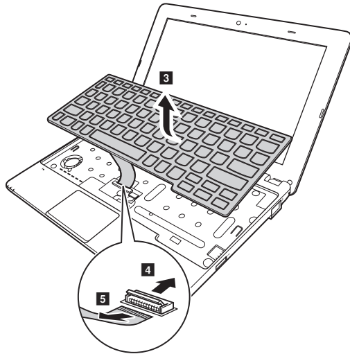
Figure 3. Removal steps of keyboard (continued)
