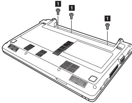
Figure 3. Removal steps of keyboard
