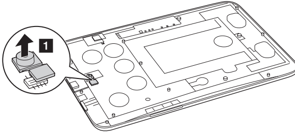
Figure 7. Removal steps of back camera
