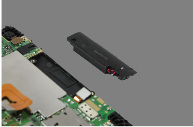
Figure 4-5. The removed speaker
