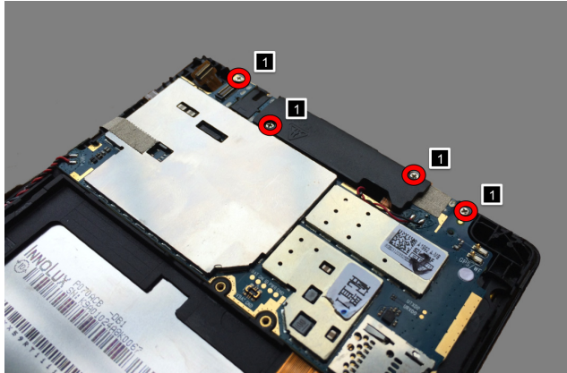
Figure 7-2. The screws on the main board assembly
