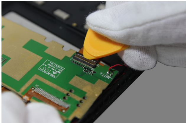
Figure 7-5. Unlocking the connector of the main FPC
