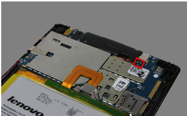
Figure 4-2. Position for desoldering the wires of the speaker (Lenovo TAB 2 A7-30F)
