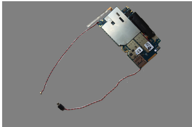
Figure 7-7. The removed main board assembly (with antenna chip, microphone, vibrator motor, speaker, side key FPC, and front camera)
