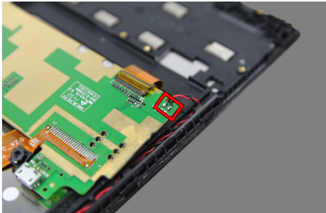
Figure 8-1. Position for desoldering the wires of the vibrator motor
