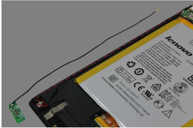
Figure 5-9. The removed antenna (Lenovo TAB 2 A7-30GC)
