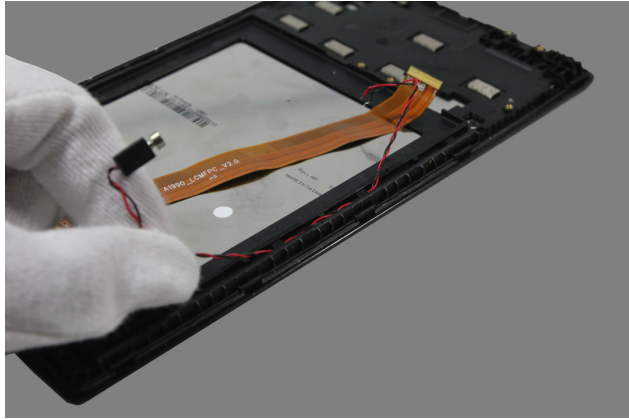
Figure 8-2. Removing the vibrator motor
