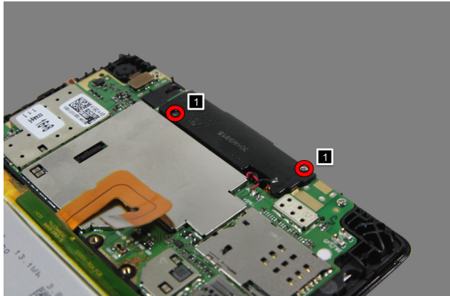
Figure 4-3. The screws on the speaker
