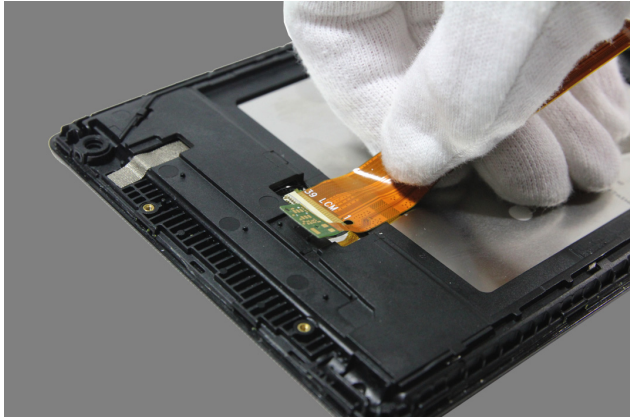
Figure 9-4. Pulling out the main FPC (from the front module side)
