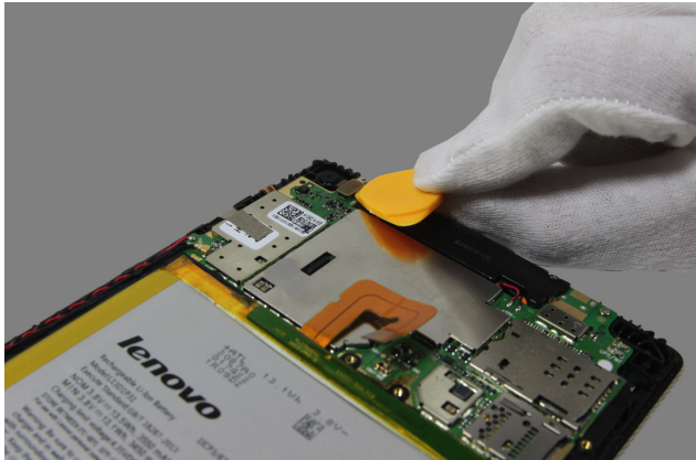
Figure 3-1. Detaching the connector of the rear camera FPC
