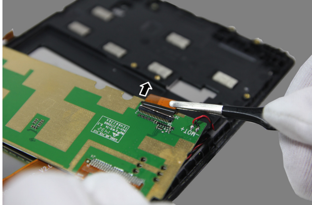
Figure 7-6. Pulling out the main FPC
