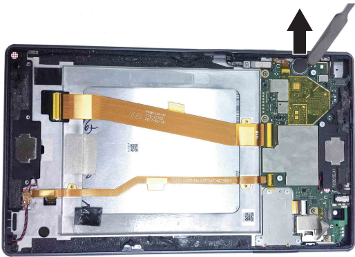
Figure 4. Removal steps of camera, motor and card slot (continued) Pry up the motor.
