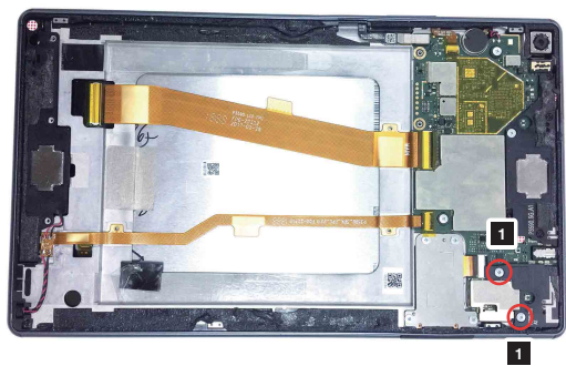
Figure 3. Removal steps of antenna bracket
