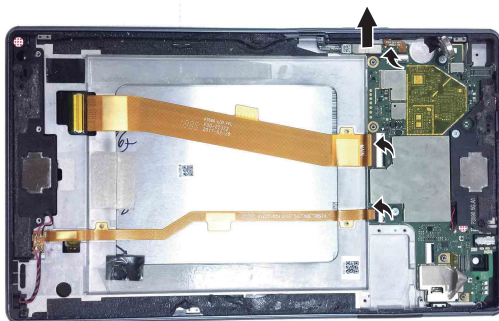
Figure 5. Removal steps of system board, speaker and microphone
