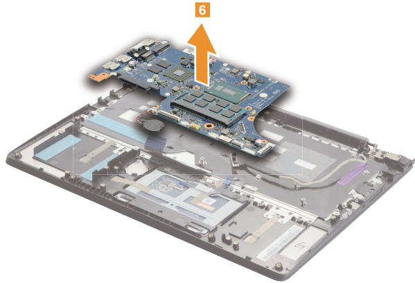
Figure 9. Removal steps of system board (continued)
