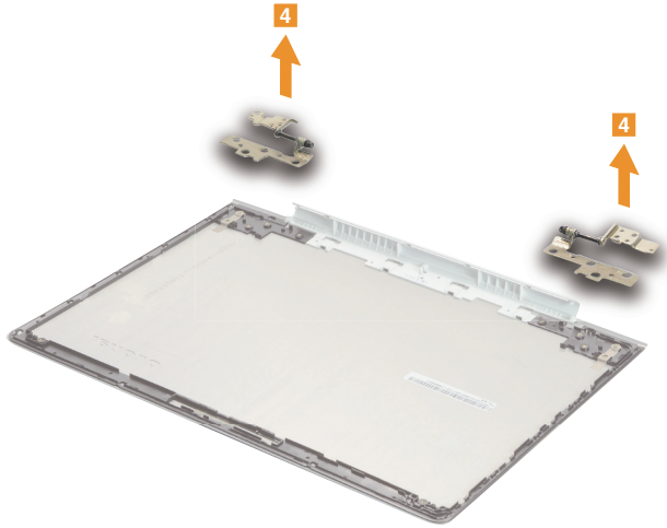
Figure 12. Removal steps of integrated camera, antenna assembly and LCD hinges (continued)
