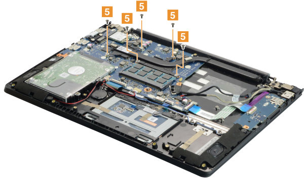
Figure 7. Removal steps of fan assembly and Heat Sink assembly (continued)
