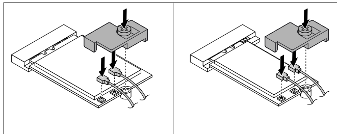
Figure 87. Connecting the Wi-Fi antenna cables and installing the Wi-Fi card shield
