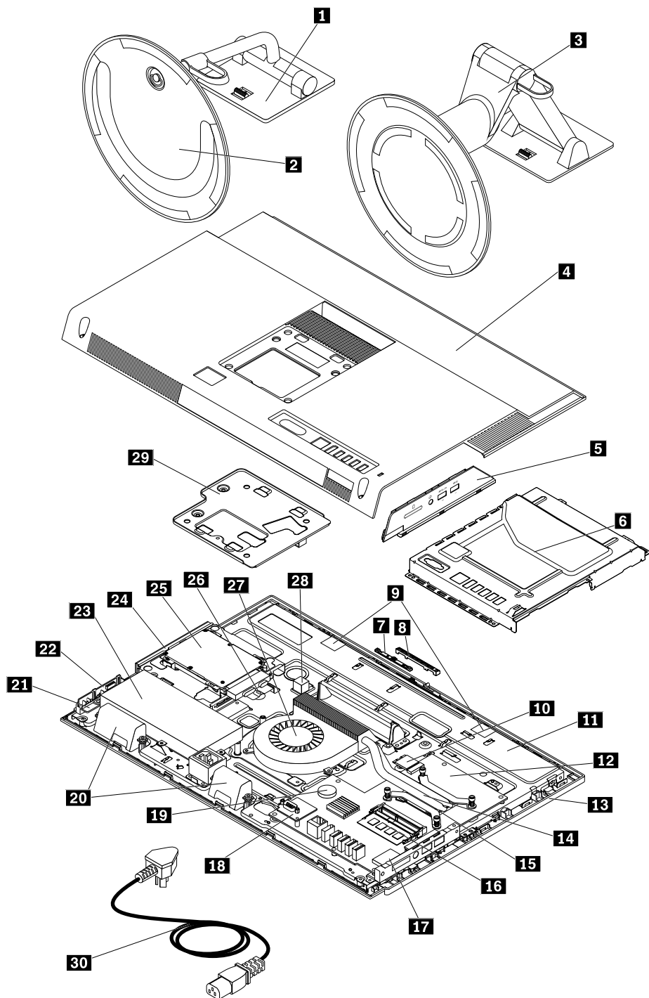
Figure 5. Computer components
