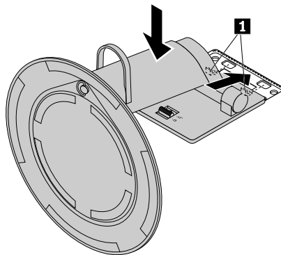
Figure 23. Installing the full-function monitor stand
