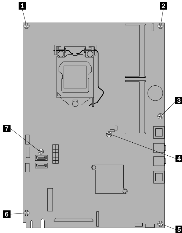
Figure 40. Removing the seven screws that secure the system board to the main bracket
