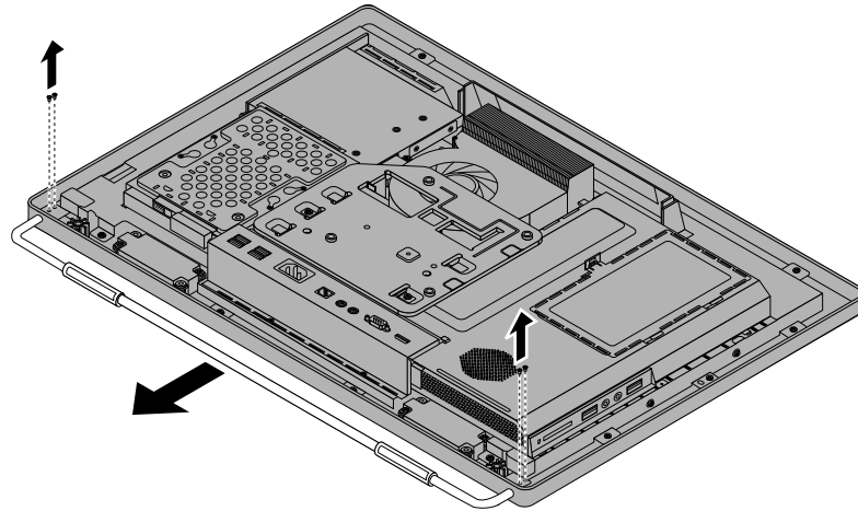
Figure 12. Removing the frame stand
