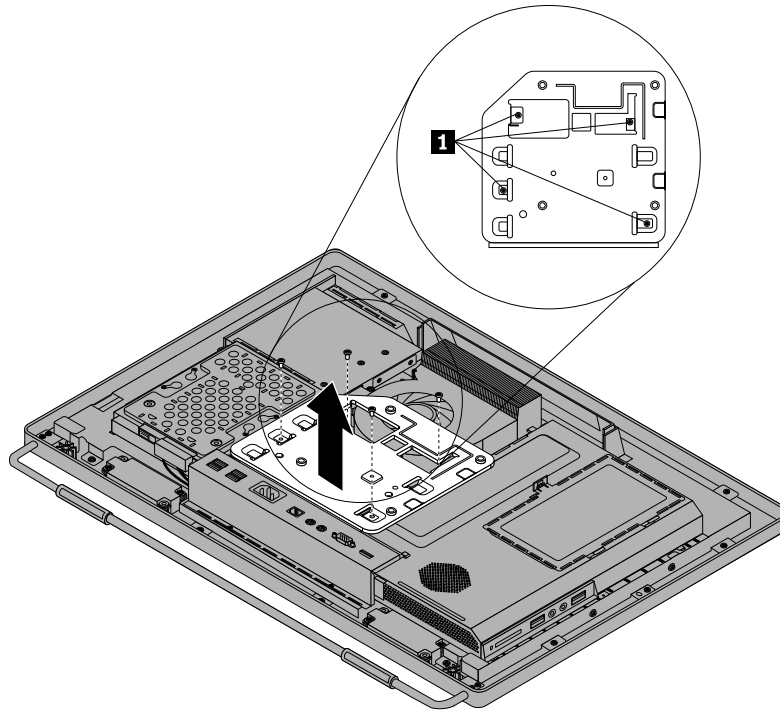
Figure 21. Removing the VESA mount bracket
