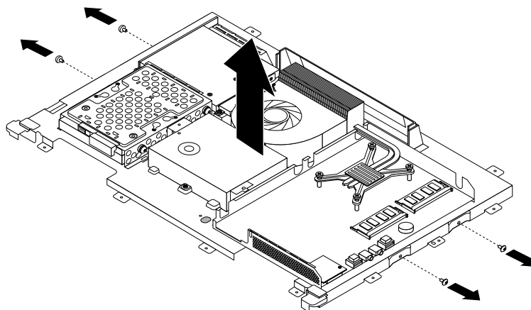
Figure 45. Removing the four screws that secure the LCD panel
