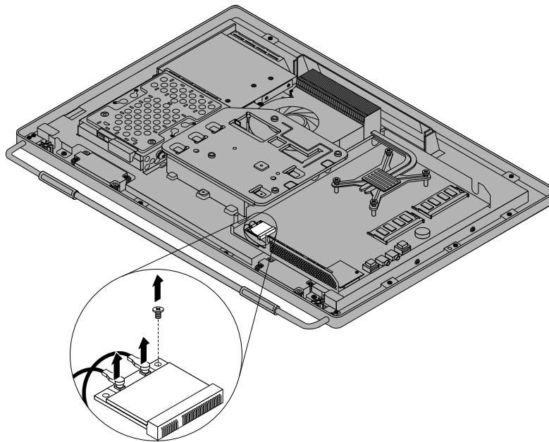
Figure 48. Removing the screw that secures the WI-FI card to the system board
