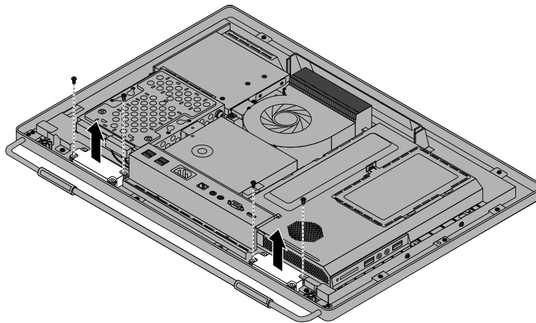
Figure 38. Removing the internal speakers
