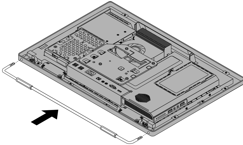
Figure 13. Reinstalling the frame stand to the computer
