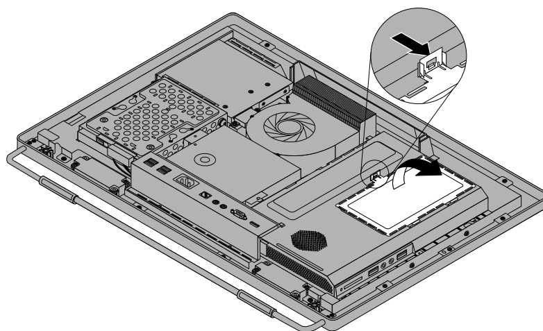
Figure 33. Opening the system board shield window
