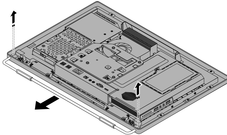
Figure 42. Removing the frame stand
