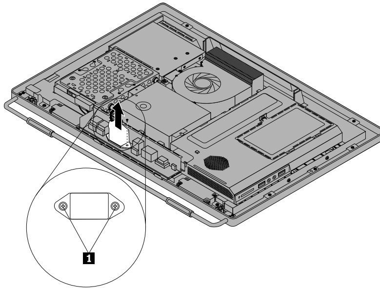
Figure 23. Removing the power cord connector
