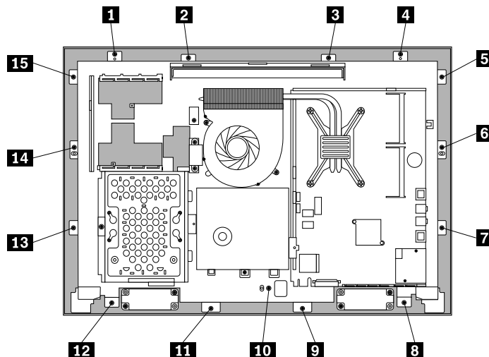
Figure 44. Removing all the 15 screws that secure the computer main bracket to the front bezel
