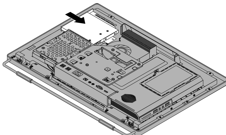
Figure 19. Installing the optical drive
