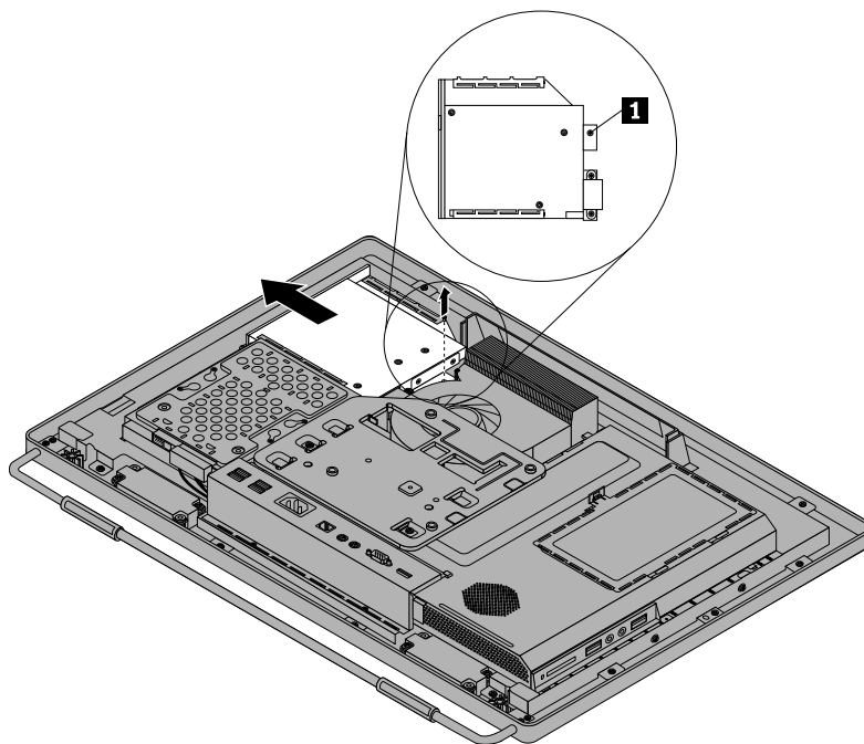
Figure 18. Removing the optical drive
