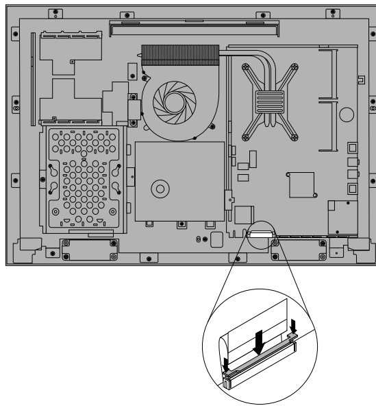
Figure 47. Reconnect the LCD panel cable to the system board
