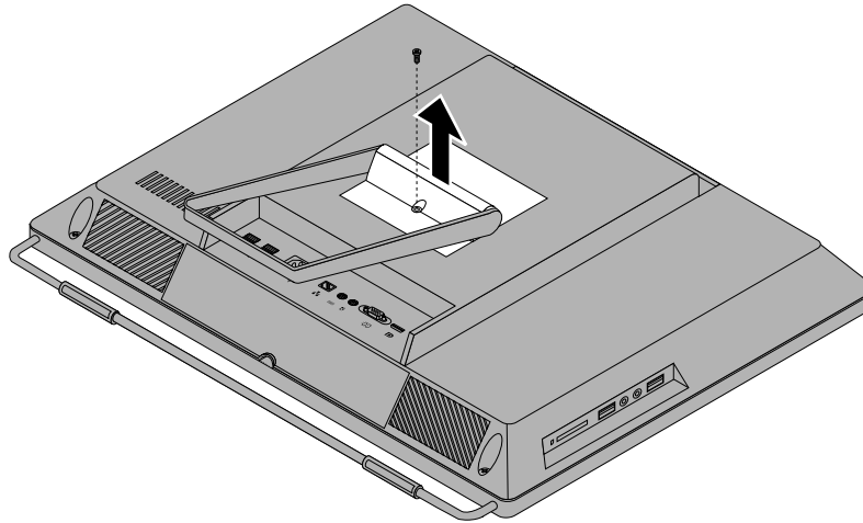
Figure 5. Removing the system stand hinge cover
