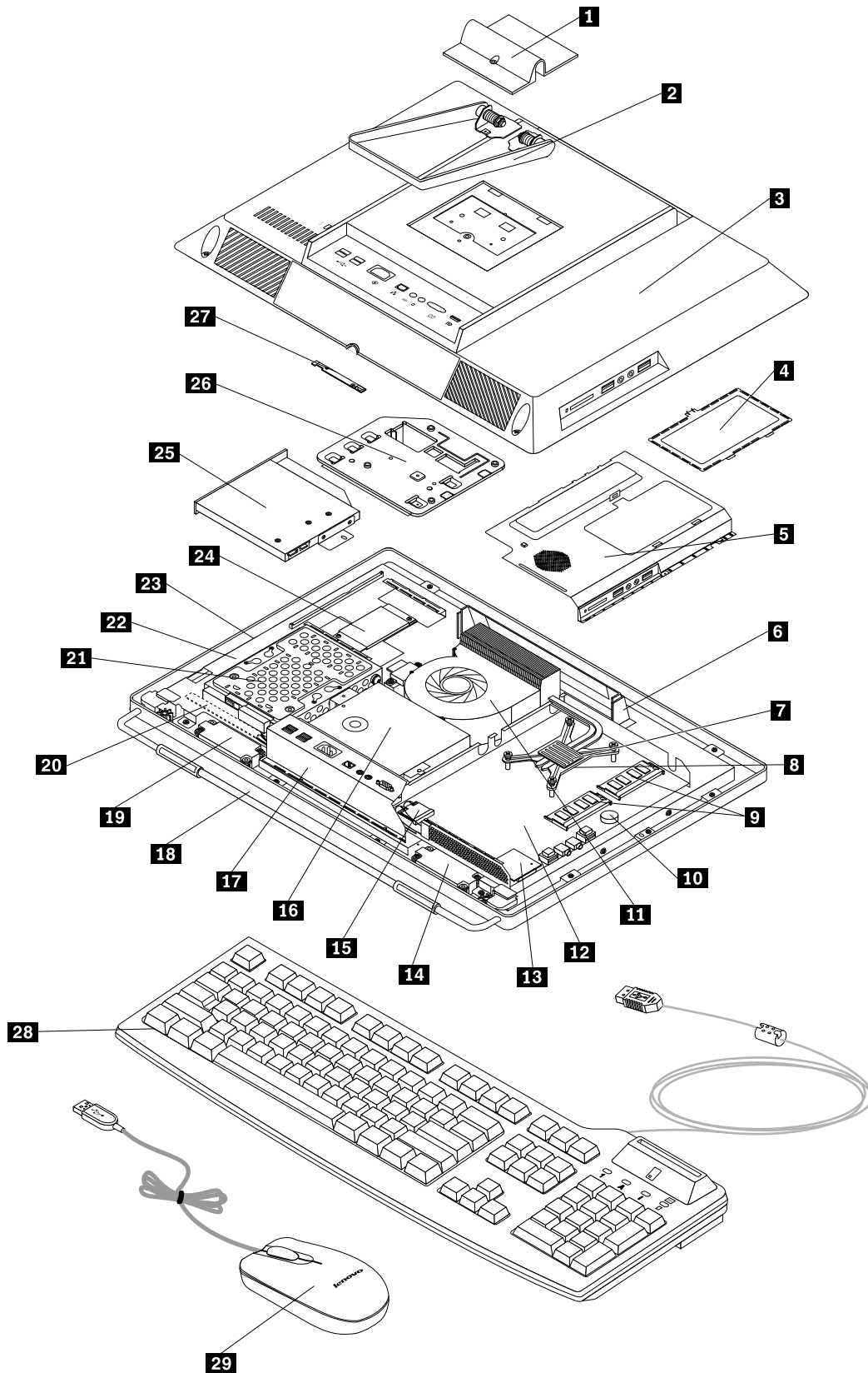
Figure 3. Locating major FRUs and CRUs
