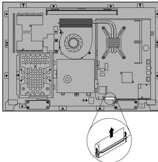
Figure 43. Disconnect the LCD panel cable from the system board
