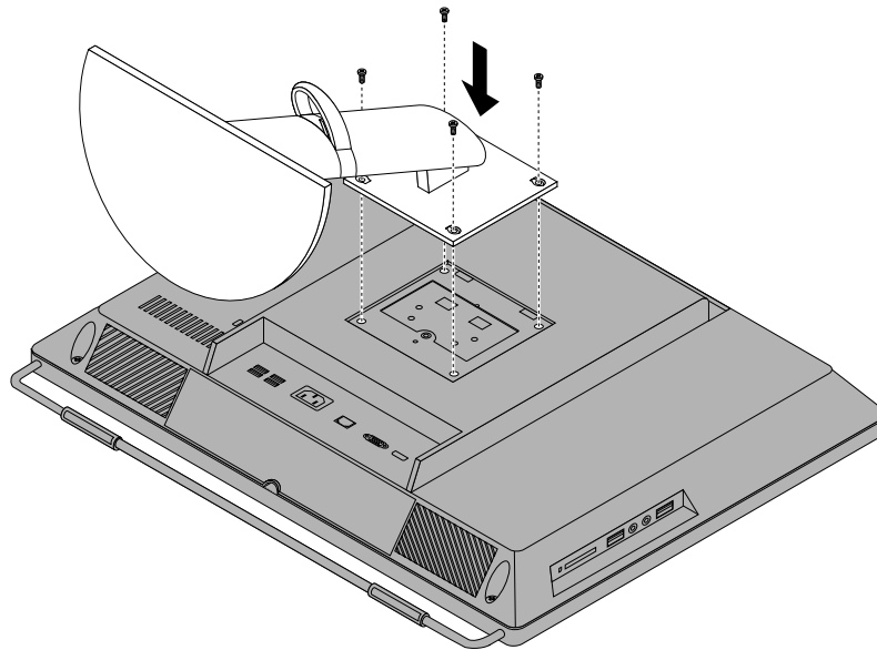
Figure 11. Reinstalling the monitor stand
