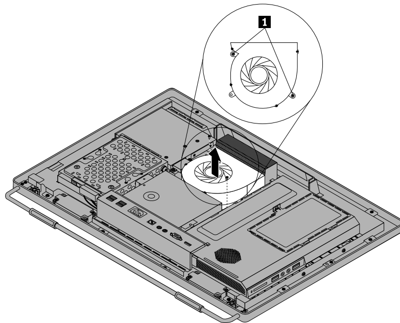
Figure 26. Removing the microprocessor fan
