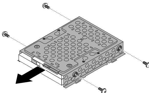
Figure 17. Removing the hard disk drive out of the bracket
