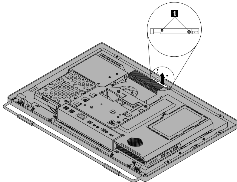
Figure 39. Removing the integrated camera
