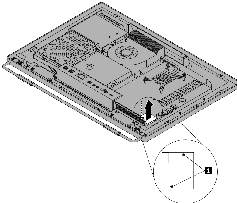
Figure 32. Removing the card reader
