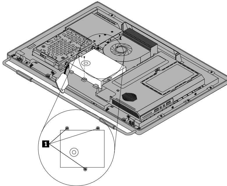
Figure 25. Removing the three screws that secure the power supply
