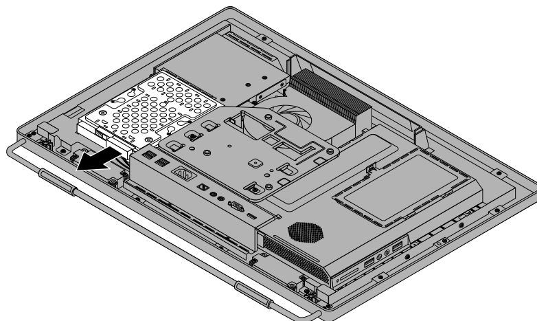
Figure 16. Removing the hard disk drive
