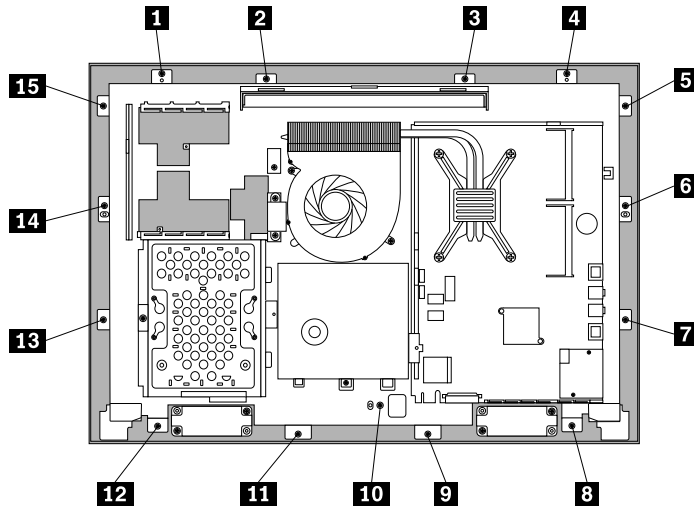
Figure 46. Reinstalling all the 15 screws that secure the computer main bracket to the front bezel
