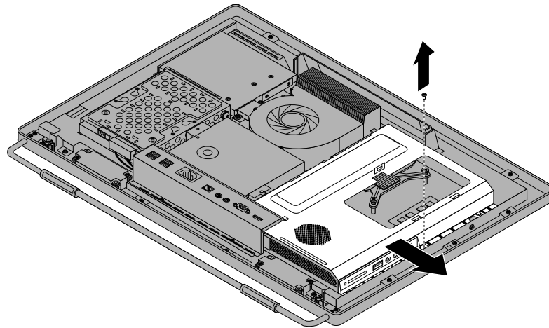
Figure 24. Removing the system board shield
