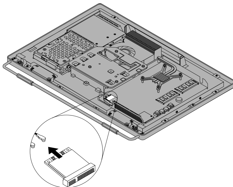
Figure 49. Removing the WI-FI card
