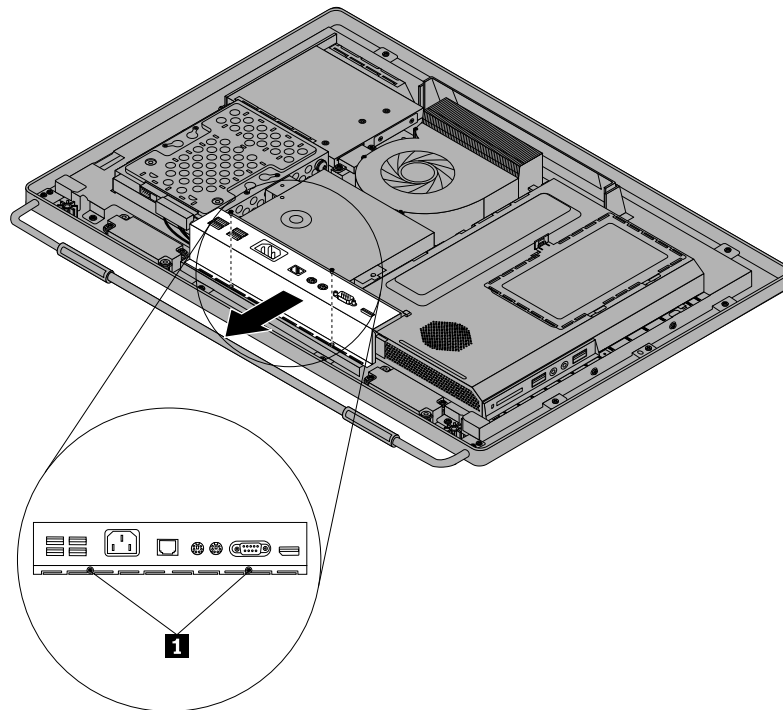
Figure 22. Removing the two screws that secure the rear I/O assembly
