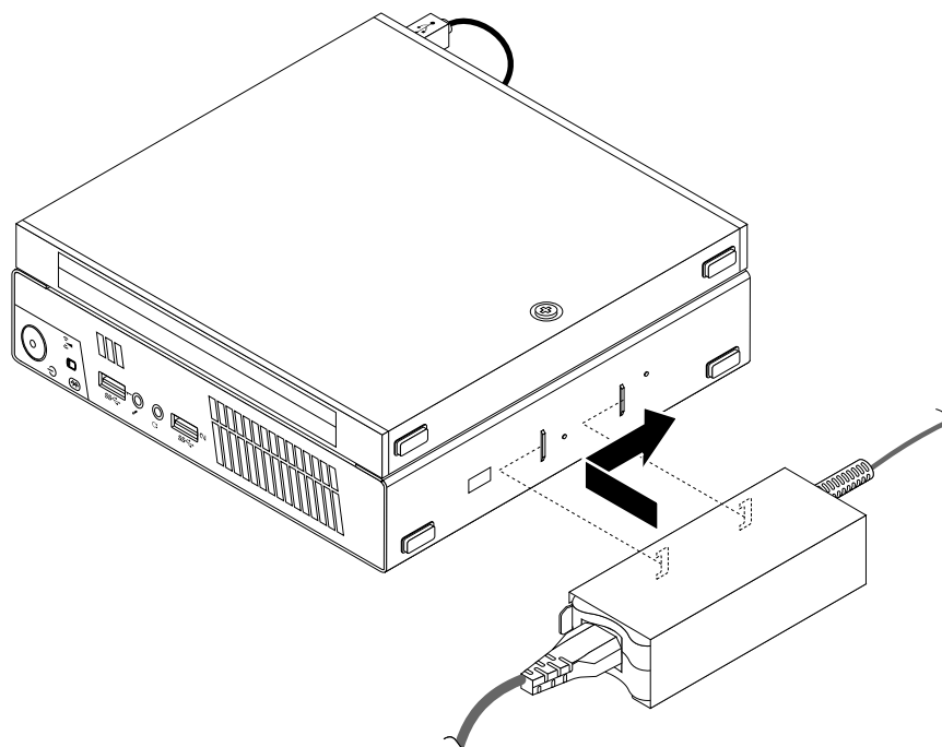
Figure 39. Installing the ac power adapter bracket
