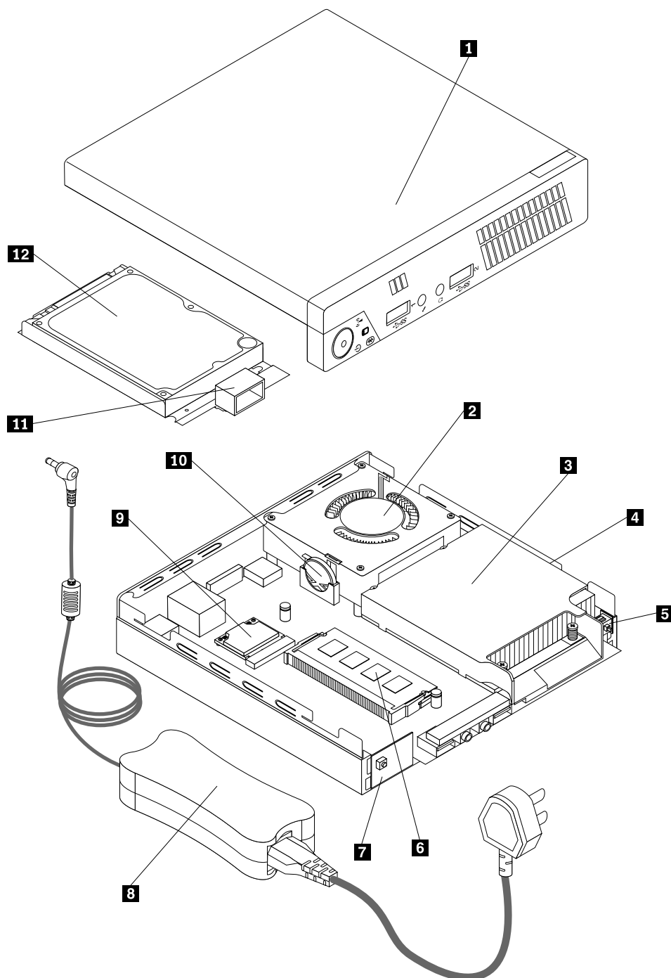
Figure 3. Component locations
