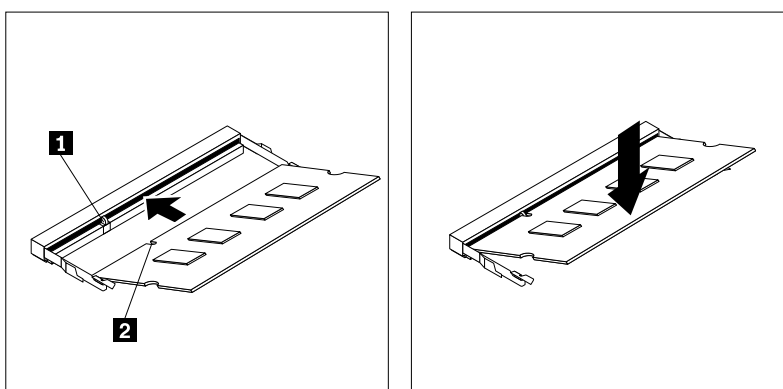
Figure 16. Installing a memory module
