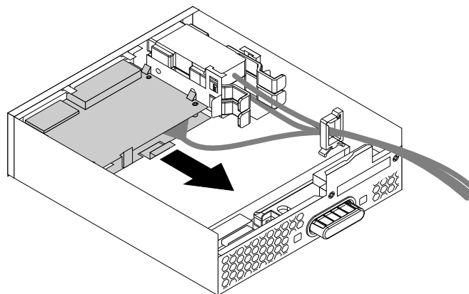
Figure 35. Removing the card reader from the flex module
