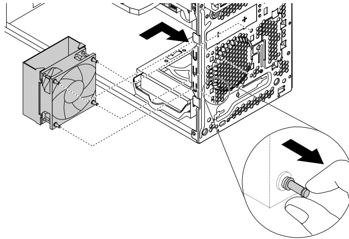
Figure 79. Installing the front fan assembly
