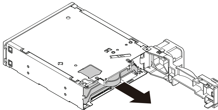
Figure 52. Removing the hard disk drive from the rear
