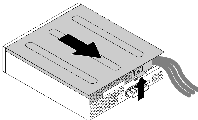
Figure 40. Removing the flex module cover
