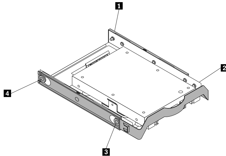
Figure 61. Installing the storage converter together with the solid-state drive into the hard-disk-drive bracket
