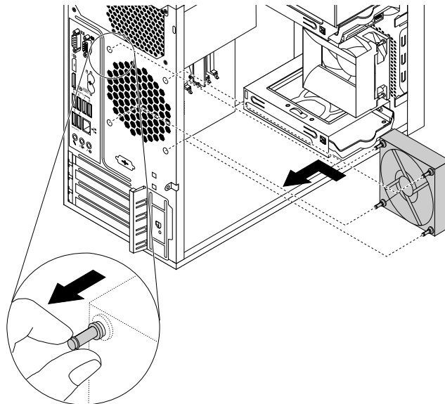
Figure 81. Installing the rear fan assembly
