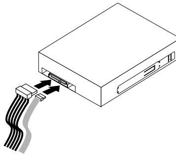
Figure 26. Connecting the cables to the rear of the new optical drive
