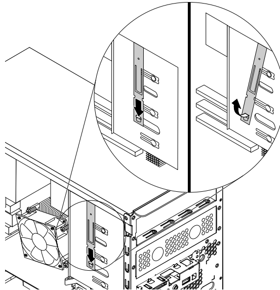
Figure 22. Removing the optical drive retainer from the computer
