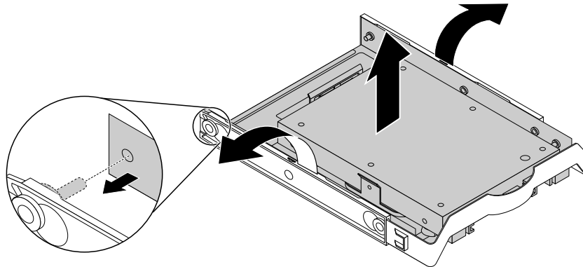
Figure 62. Removing the storage converter from the 3.5-inch hard-disk-drive bracket
