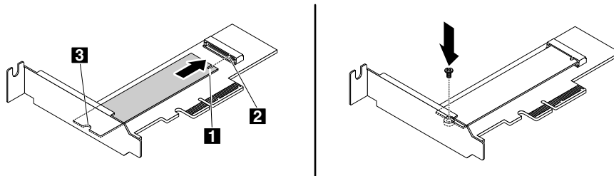
Figure 17. Installing the M.2 solid-state drive
