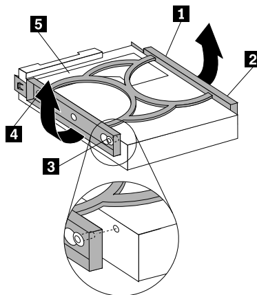
Figure 67. Installing the hard disk drive into the bracket
