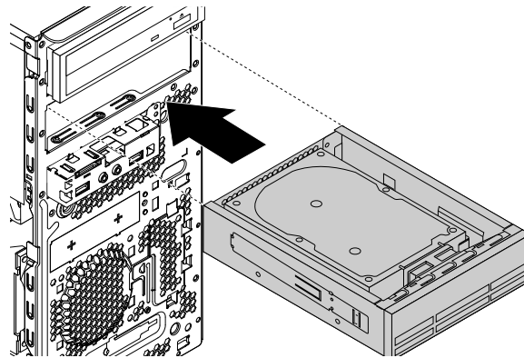
Figure 76. Installing the optical drive bracket
