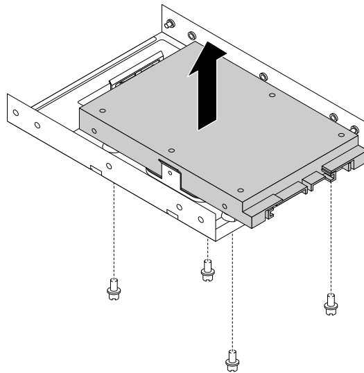
Figure 63. Removing the solid-state drive from the storage converter
