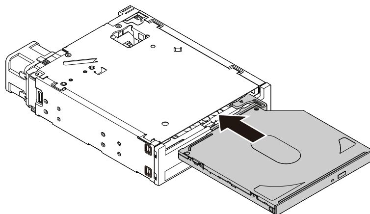
Figure 50. Installing the slim optical drive in the enclosure
