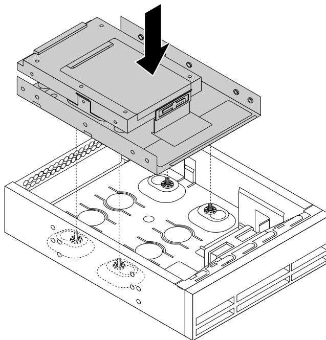
Figure 74. Installing the solid-state drive with the storage converter
