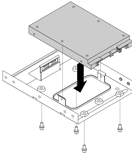
Figure 64. Installing the new solid-state drive into the storage converter
