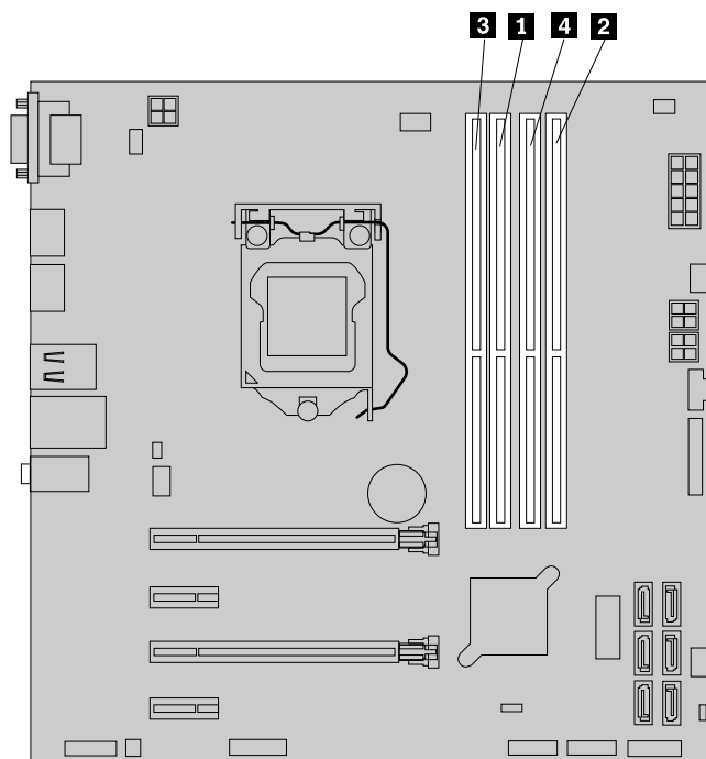
Figure 18. Memory module installation—order
