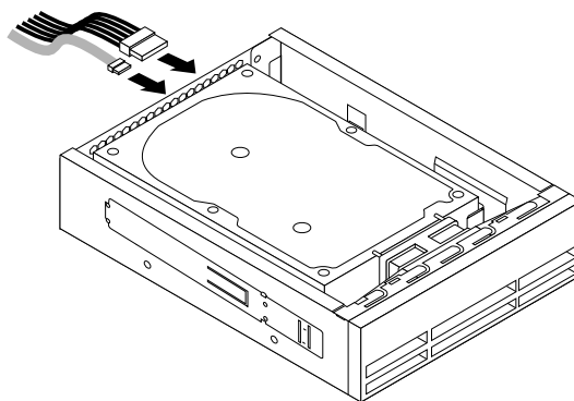
Figure 77. Connecting the hard disk drive or solid-state drive
