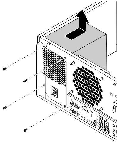
Figure 58. Removing the screws for the power supply assembly
