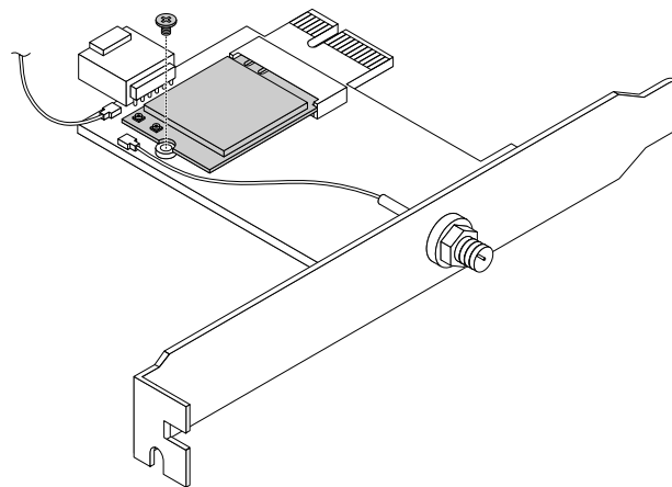
Figure 86. Removing the screw that secures the Wi-Fi card module
