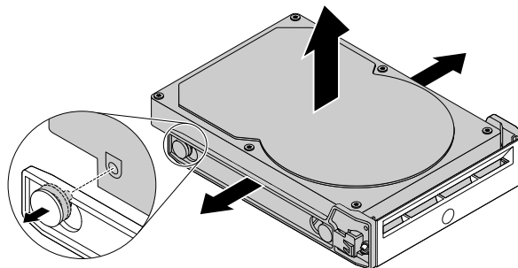
Figure 46. Removing the hard disk drive from the bracket
