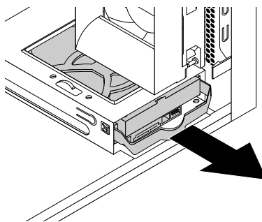
Figure 69. Removing the secondary hard disk drive
