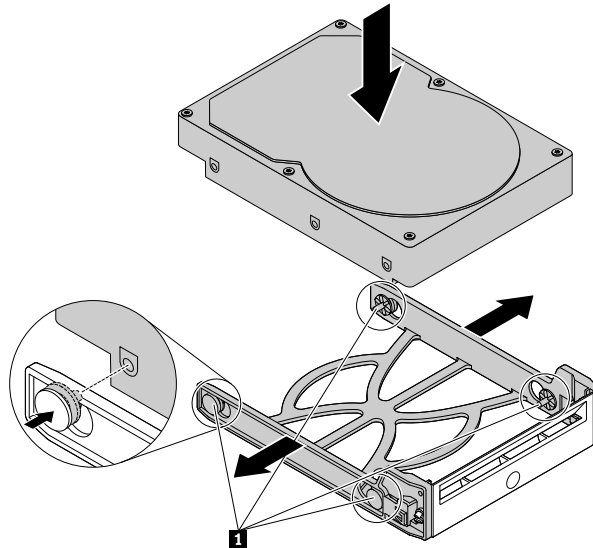
Figure 47. Installing the hard disk drive into the bracket
