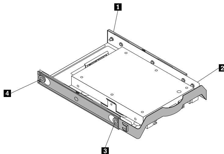
Figure 65. Installing the storage converter with the new solid-state drive into the hard-disk-drive bracket
