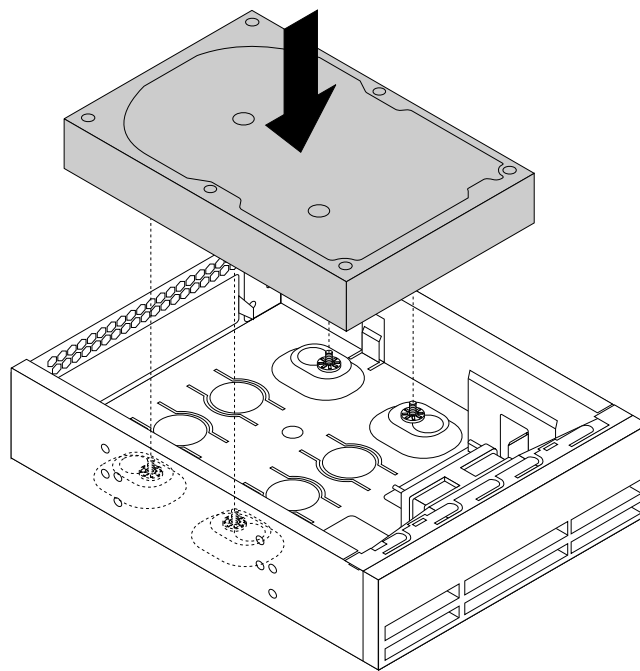
Figure 72. Installing the tertiary hard disk drive
