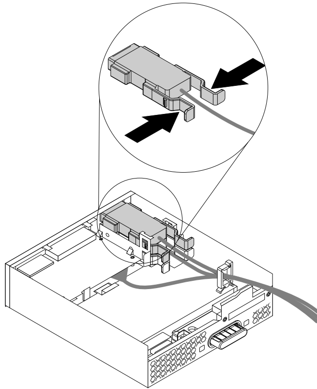
Figure 41. Removing the eSATA connector or IEEE 1394 connector from the flex module
