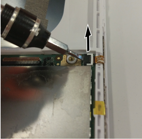
Figure 6. Removal steps of sidekey
