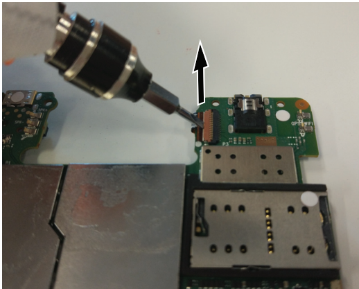
Figure 9. Removal steps of front camera
