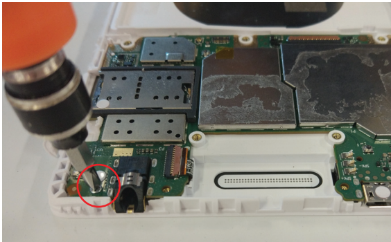
Figure 8. Removal steps of main board
