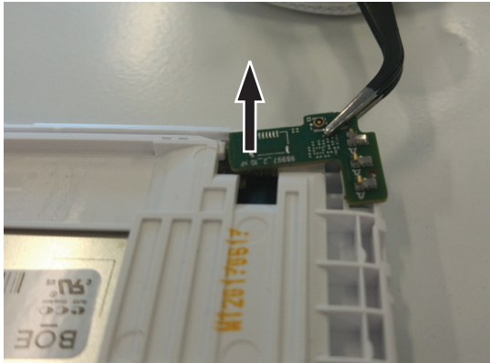
Figure 3. Removal steps of sub board (continued)
