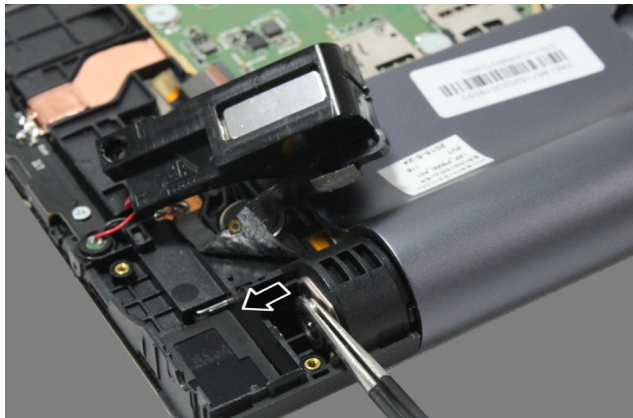
Figure 6-3. Pulling out the hinge pivot
