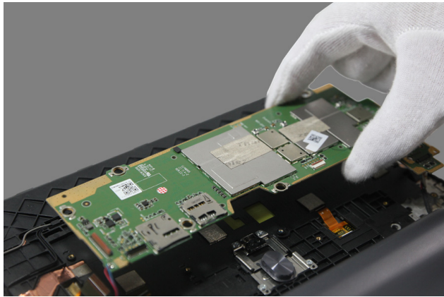
Figure 15-3. Detaching the main board
