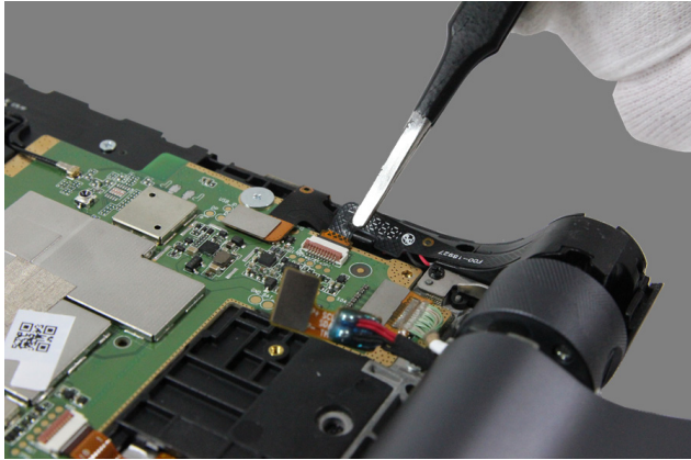
Figure 3-8. Pulling out the power key FPC
