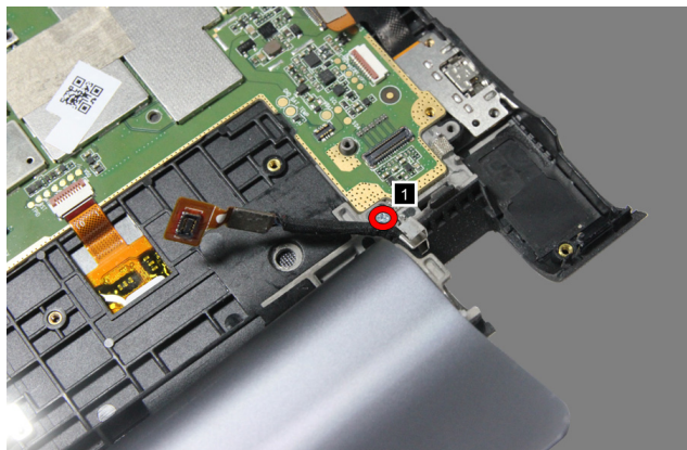
Figure 6-1. The screws on the metal piece for fastening the battery and camera FPC
