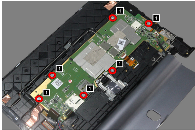
Figure 10-2. The screws on the main board
