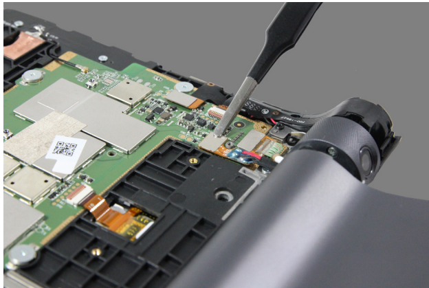
Figure 2-3. Disconnecting the power supply of the tablet
