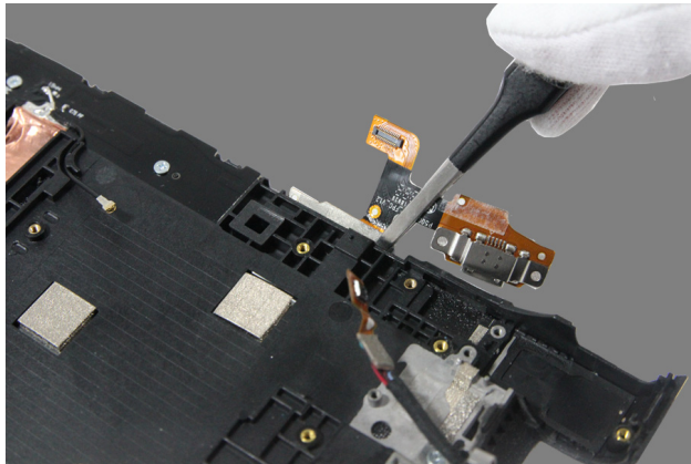
Figure 10-5. Detaching the USB and volume key FPC
