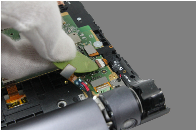
Figure 2-7. Unlocking the connector of the power key FPC
