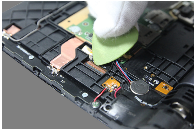
Figure 7-3. Unlocking the connector of the LCD FPC (front module side)
