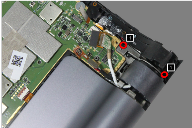
Figure 2-4. The screws on the holder of the rotated camera
