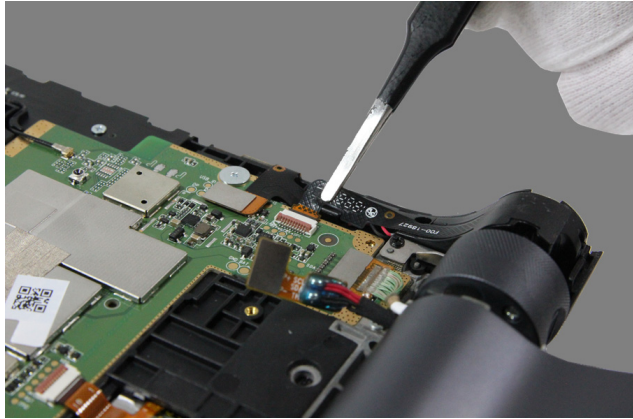
Figure 2-8. Pulling out the power key FPC
