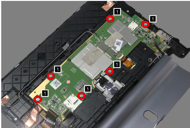
Figure 13-3. The screws on the main board
