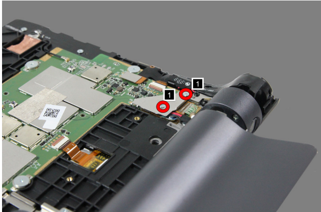
Figure 2-1. The screws on the metal piece for fixing the battery FPC
