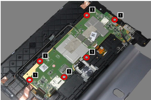
Figure 15-2. The screws on the main board
