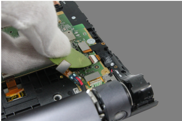
Figure 3-7. Unlocking the connector of the power key FPC
