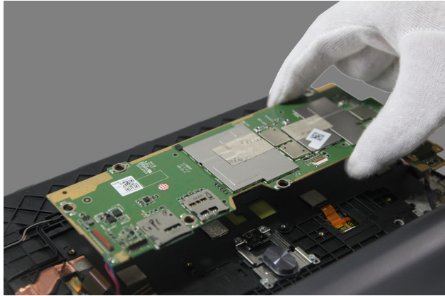
Figure 13-4. Detaching the main board
