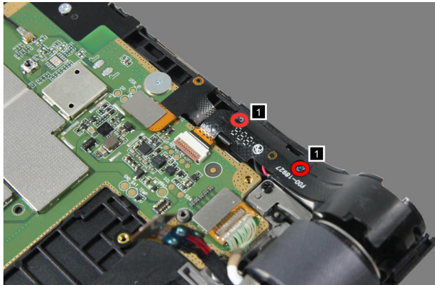
Figure 2-5. The screws on the left speaker unit
