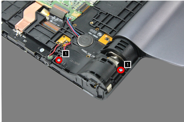
Figure 5-1. The screws on the right speaker
