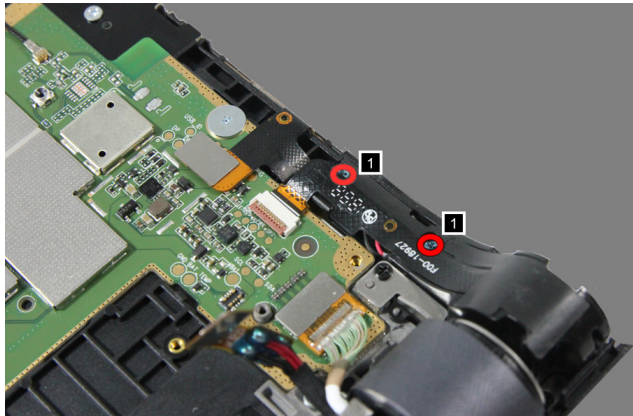
Figure 3-5. The screws on the left speaker unit
