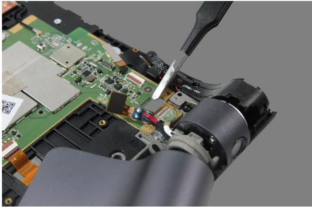
Figure 2-6. Detaching the FPC connector of the rotated camera
