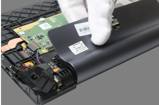
Figure 6-4. Detaching the battery pack at the left end
