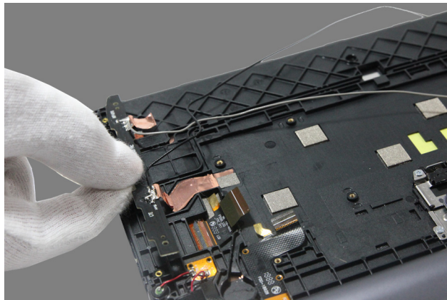
Figure 13-5. Removing the antenna
