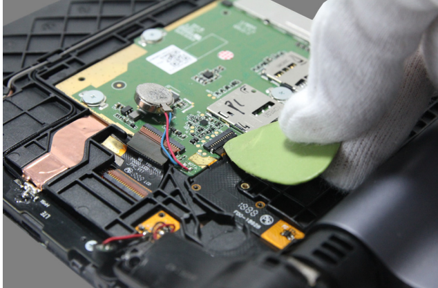
Figure 5-4. Unlocking the connector of the right speaker FPC
