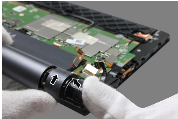
Figure 2-9. Removing the left speaker assembly unit (with power key FPC)
