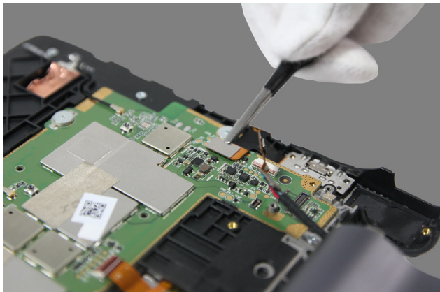
Figure 9-3. Detaching the connector of the USB and volume key FPC
