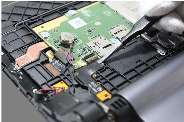
Figure 5-5. Pulling out the right speaker FPC
