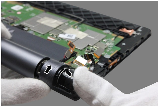
Figure 3-9. Removing the rotated camera
