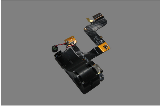
Figure 5-6. The removed right speaker assembly unit (with microphone and audio jack)
