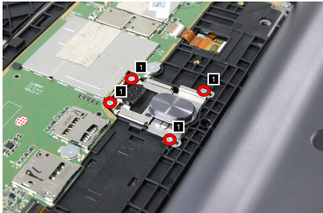
Figure 4-1. The screws on the hinge latch
