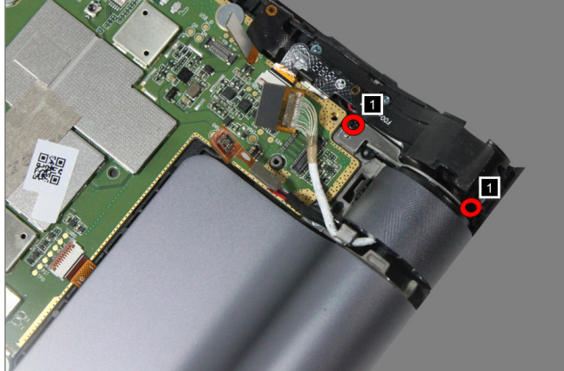
Figure 3-4. The screws on the holder of the rotated camera
