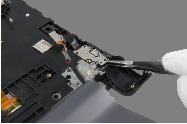
Figure 10-4. Detaching the USB and volume key FPC from its seat
