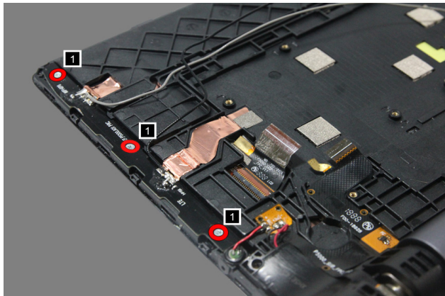
Figure 13-1. The screw on the antenna
