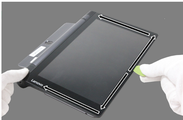
Figure 1-4. Unlocking the rear cover from the main body (along the joint line)
