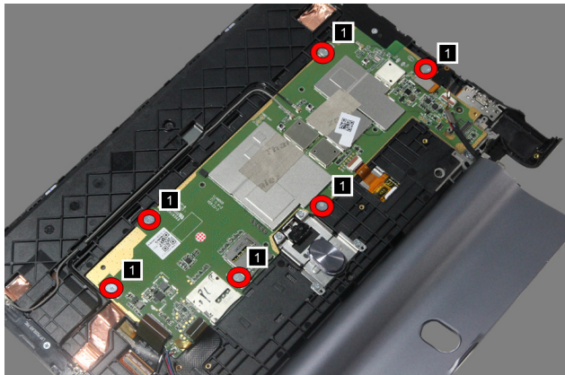
Figure 9-5. The screws on the main board
