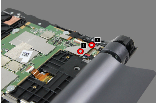
Figure 3-1. The screws on the metal piece for fixing the battery FPC
