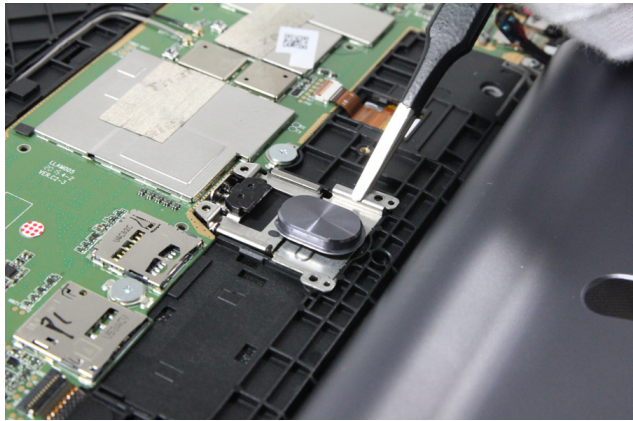
Figure 4-2. Removing the hinge frame latch
