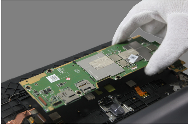
Figure 9-6. Removing the main board
