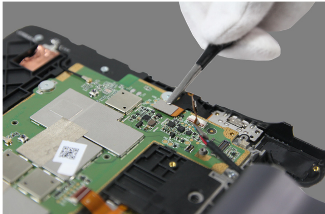
Figure 10-1. Detaching the connector of the USB and volume key FPC
