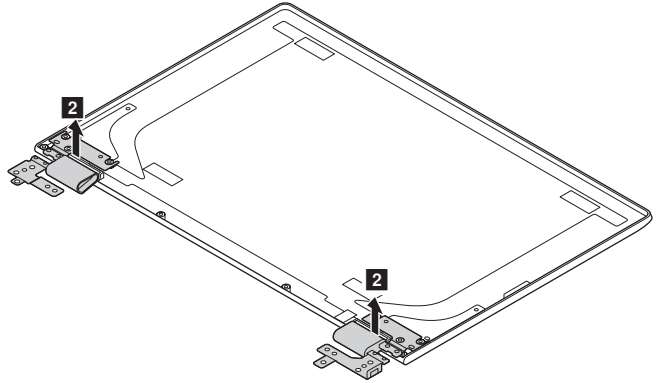
Figure 13. Removal steps of LCD unit (continued)
