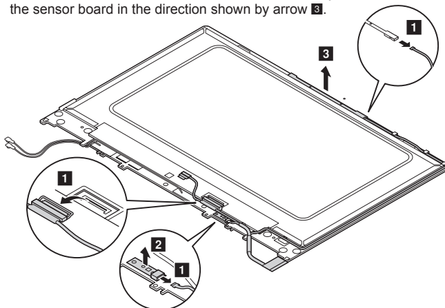
Figure 14. Removal steps of MIC board, sensor board and camera
