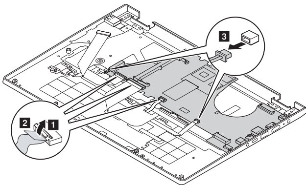
Figure 9. Removal steps of system board
