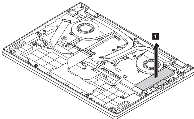
Figure 5. Removal steps of SSD card
