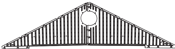
*AGQ (x8) Roof Panel
