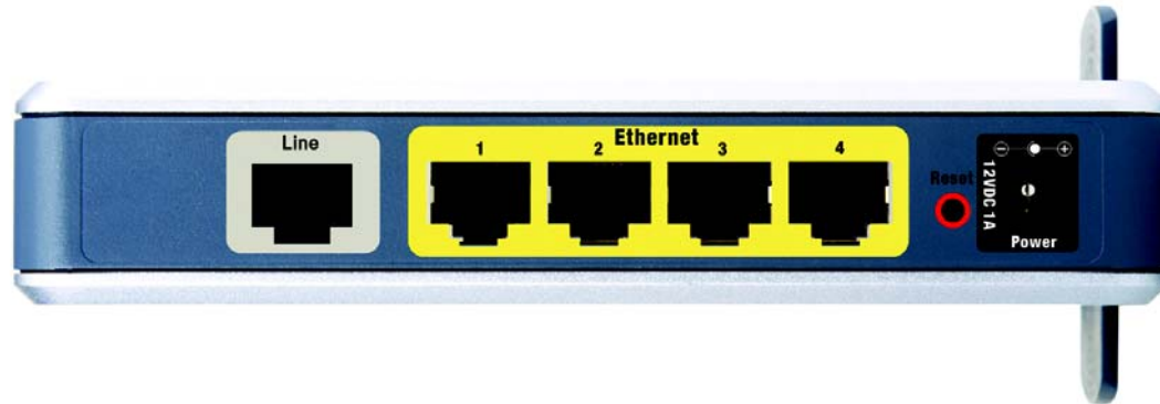
Figure 3-1: Ports and Reset Button on Side Panel
