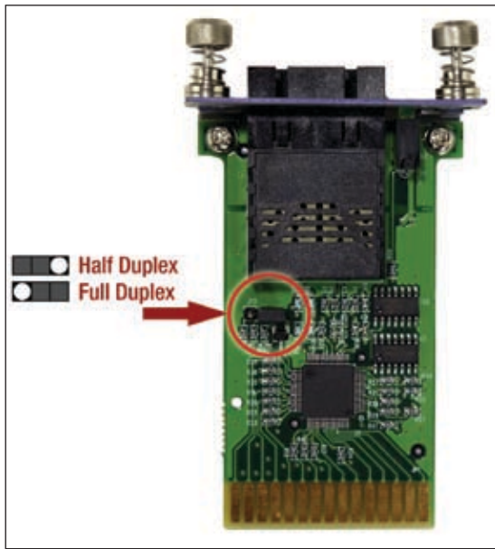
Jumper Diagram
