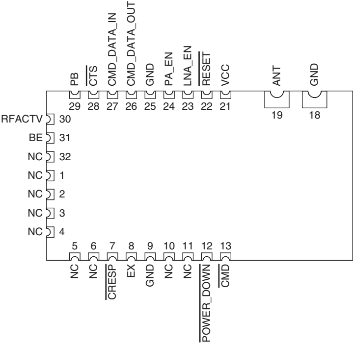
Figure 28: HumRC™ Series Transceiver Pre-certified Version Pin Assignments (Top View)
