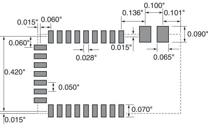
Figure 50: HUM-***-RC-UFL/GAS Recommended PCB Layout
