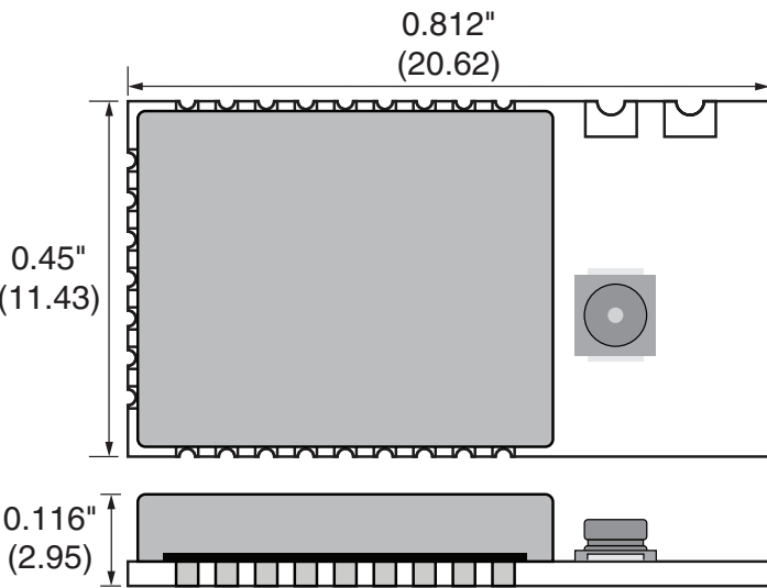
Figure 30: HumRC™ Series Transceiver Pre-certified Version Dimensions
