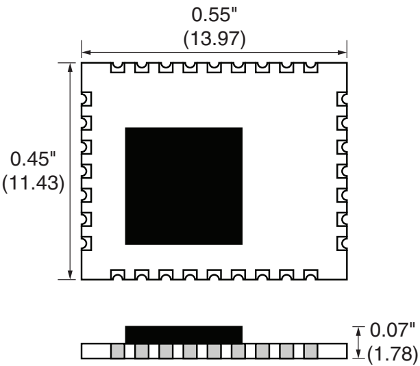
Figure 29: HumRC™ Series Transceiver Dimensions
