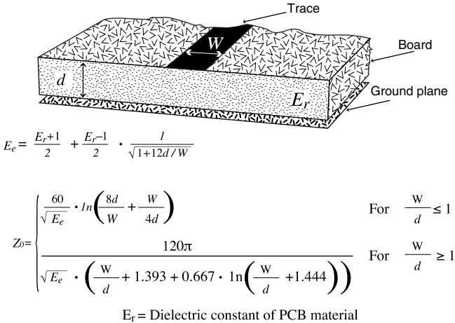
Figure 51: Microstrip Formulas
