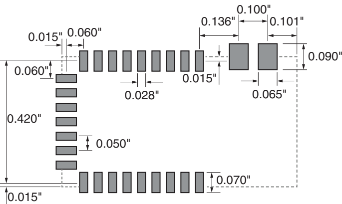
Figure 51: HUM-***-RC-UFL/GAS Recommended PCB Layout
