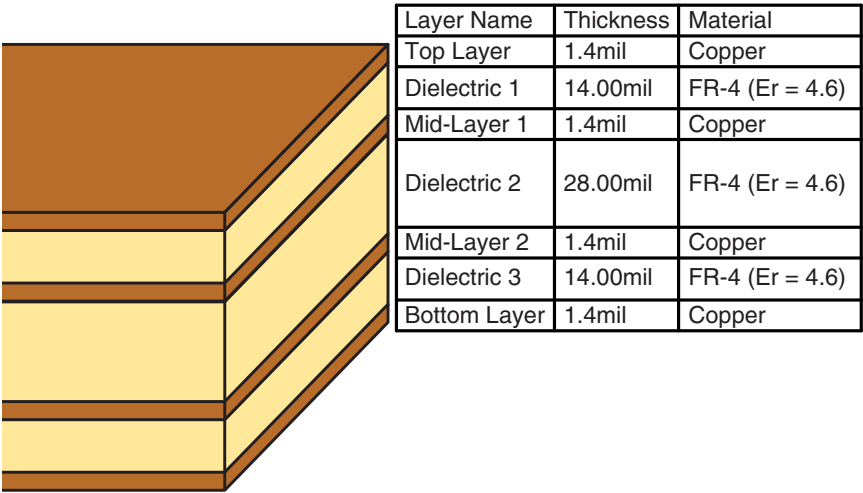
Figure 46: HumRC™ Series Transceiver Castellation Version Reference Design PCB Stack
