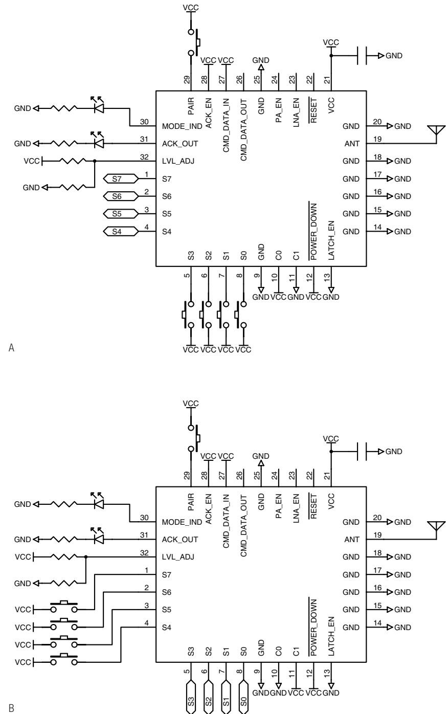
Figure 42: HumRC™ Series Transceiver Basic Application Circuits for Bi-directional Remote Control
