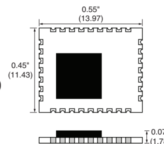
Figure 1: Package Dimensions
