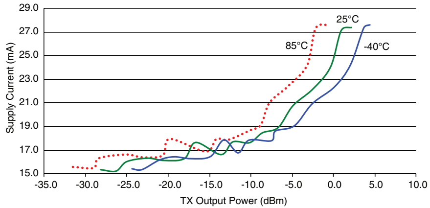
Figure 10: HumRC™ Series Transceiver Average Current vs. Transmitter Output Power at 2.5V - HUM-2.4-RC
