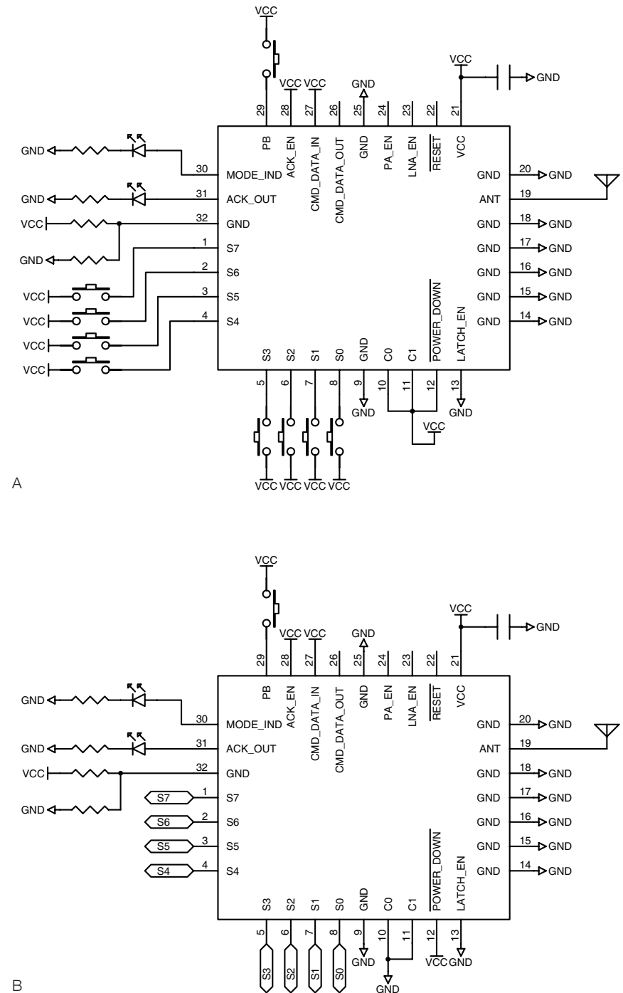
Figure 86: HumPRC™ Series Transceiver Basic Application Circuits for Remote Control
