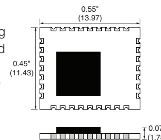
Figure 1: Package Dimensions
