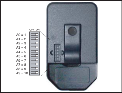
Figure 2: DIP Switch Assignments
