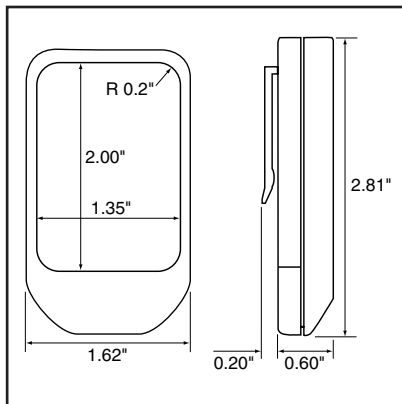
Figure 1: Physical Dimensions
