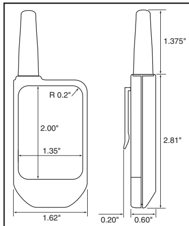
Figure 1: Physical Dimensions
